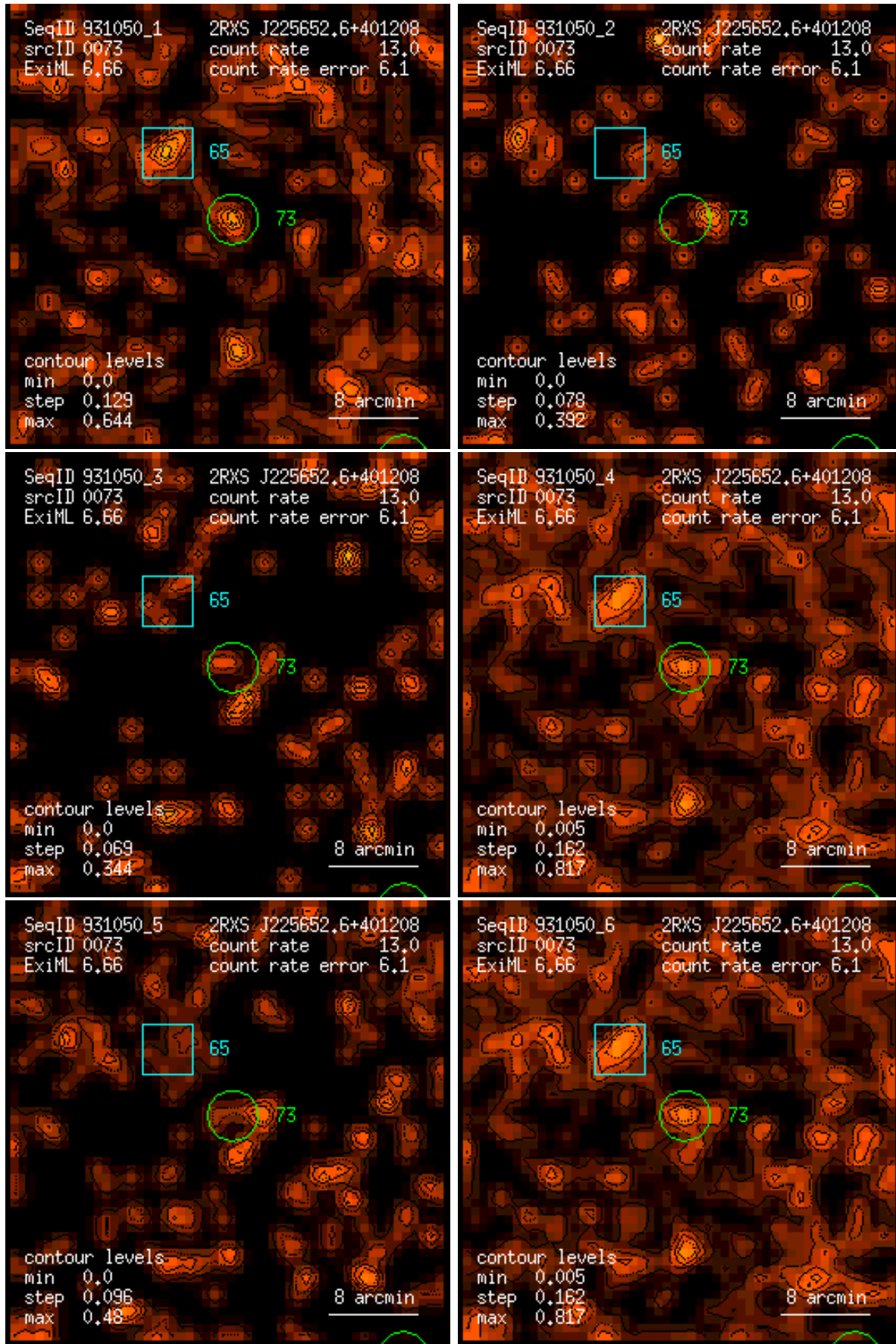
Figure 73: RASS 931050: detection 0073: band rate images, Gaussian filter: (1) PSPC channels 11 – 41, (2) 52 – 90, (3) 91 – 201, (4) 11 – 235, (5) 52 – 201, (6) 11 – 201. Broad band rates in counts/ks. Band rate contour levels in counts/ks/arcmin 2 .
