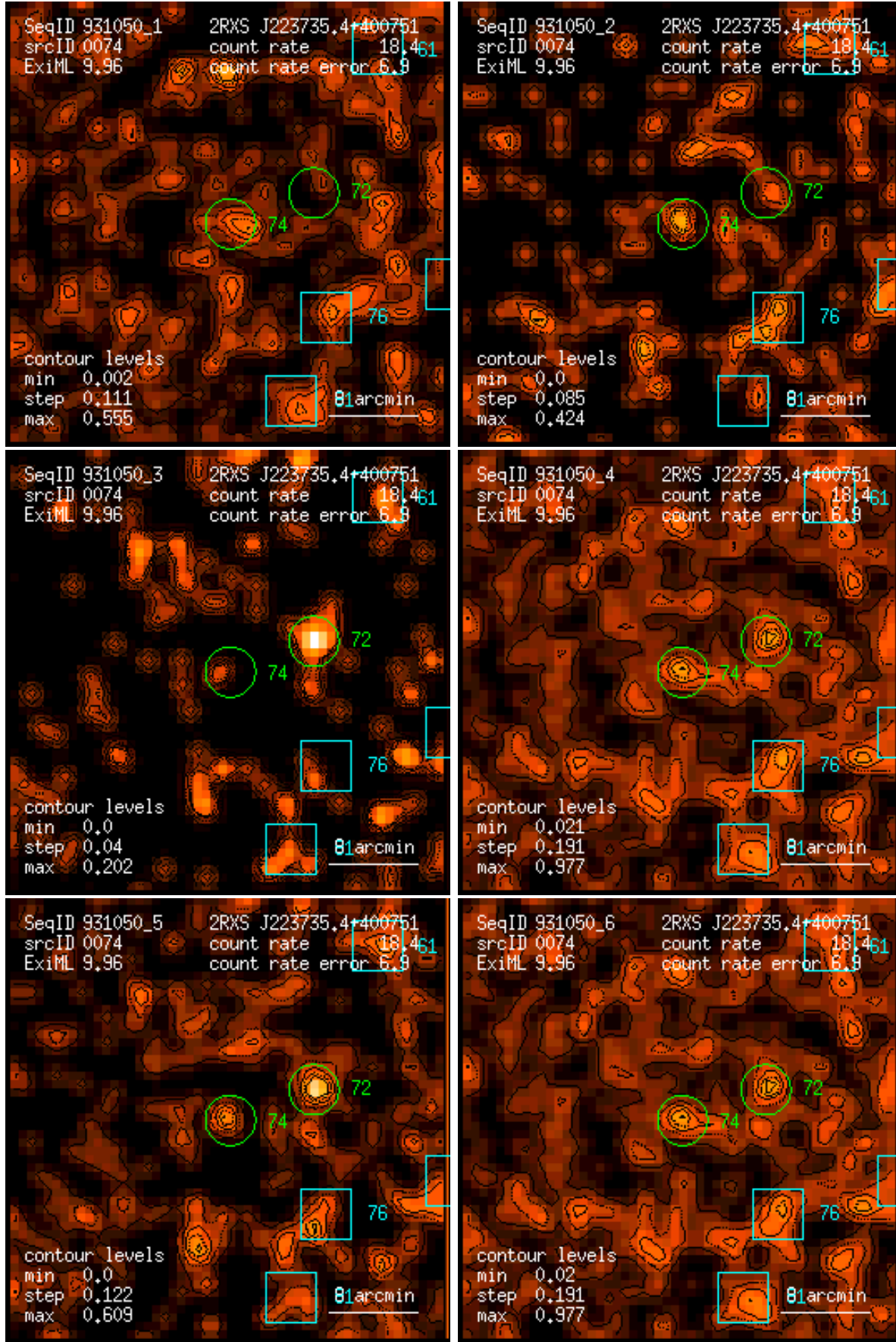
Figure 74: RASS 931050: detection 0074: band rate images, Gaussian filter: (1) PSPC channels 11 – 41, (2) 52 – 90, (3) 91 – 201, (4) 11 – 235, (5) 52 – 201, (6) 11 – 201. Broad band rates in counts/ks. Band rate contour levels in counts/ks/arcmin 2 .
