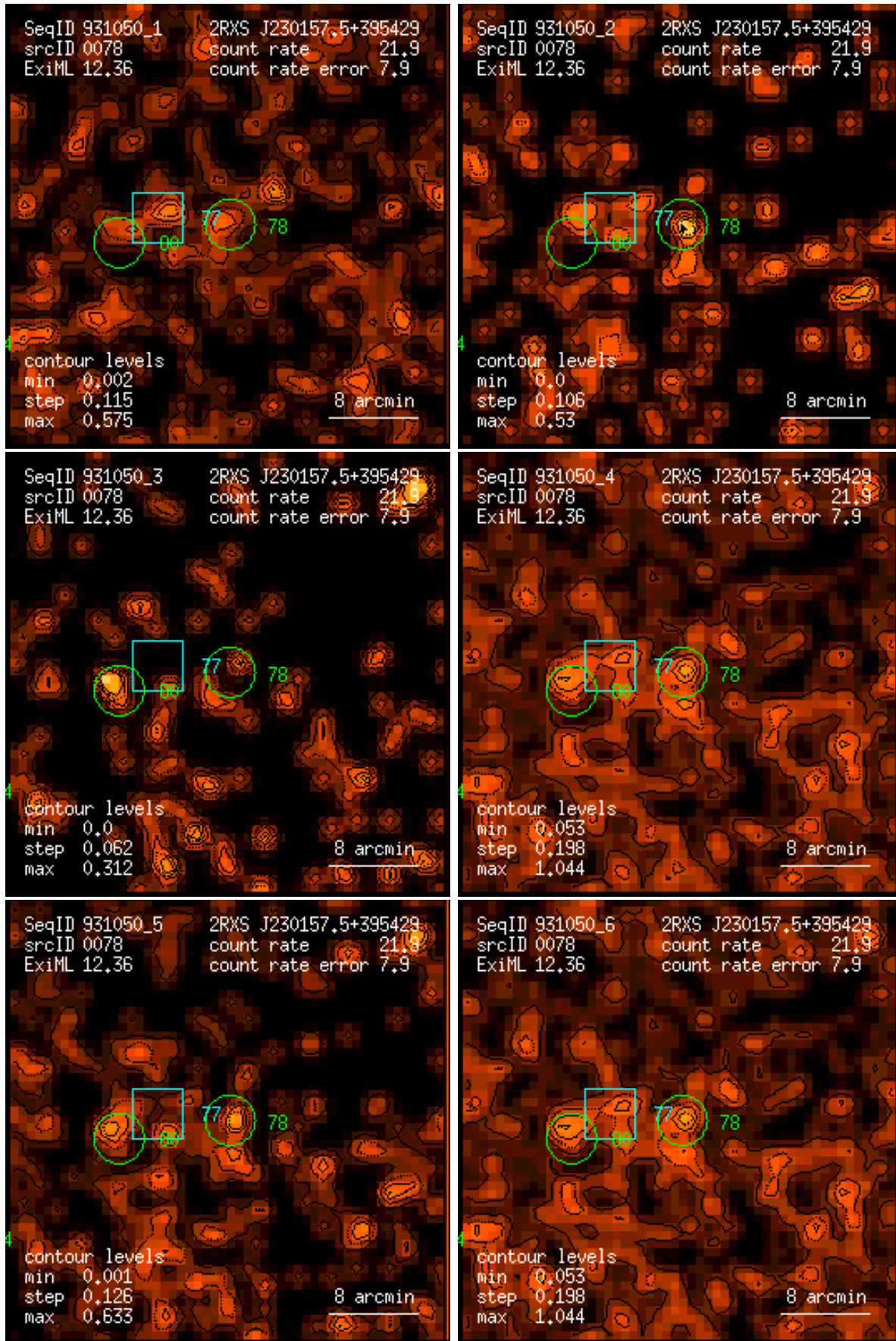
Figure 78: RASS 931050: detection 0078: band rate images, Gaussian filter: (1) PSPC channels 11 – 41, (2) 52 – 90, (3) 91 – 201, (4) 11 – 235, (5) 52 – 201, (6) 11 – 201. Broad band rates in counts/ks. Band rate contour levels in counts/ks/arcmin 2 .
