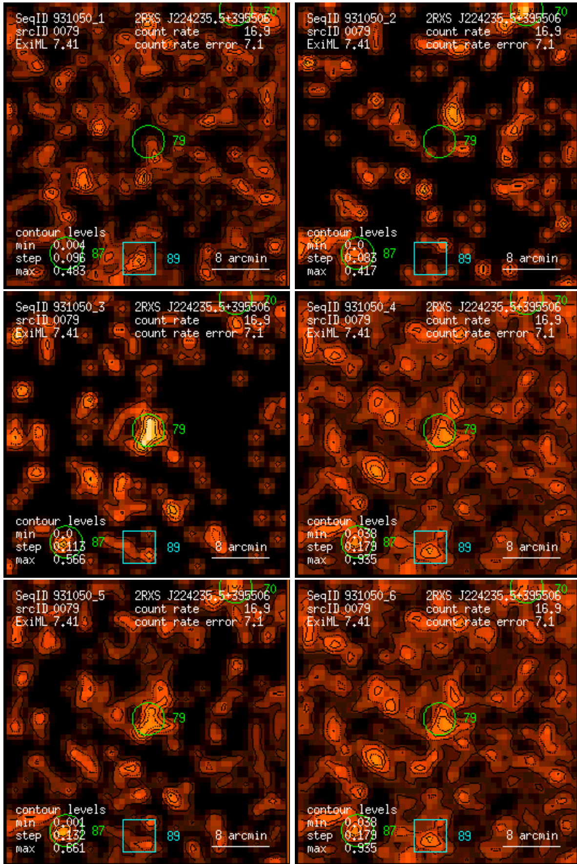
Figure 79: RASS 931050: detection 0079: band rate images, Gaussian filter: (1) PSPC channels 11 – 41, (2) 52 – 90, (3) 91 – 201, (4) 11 – 235, (5) 52 – 201, (6) 11 – 201. Broad band rates in counts/ks. Band rate contour levels in counts/ks/arcmin 2 .
