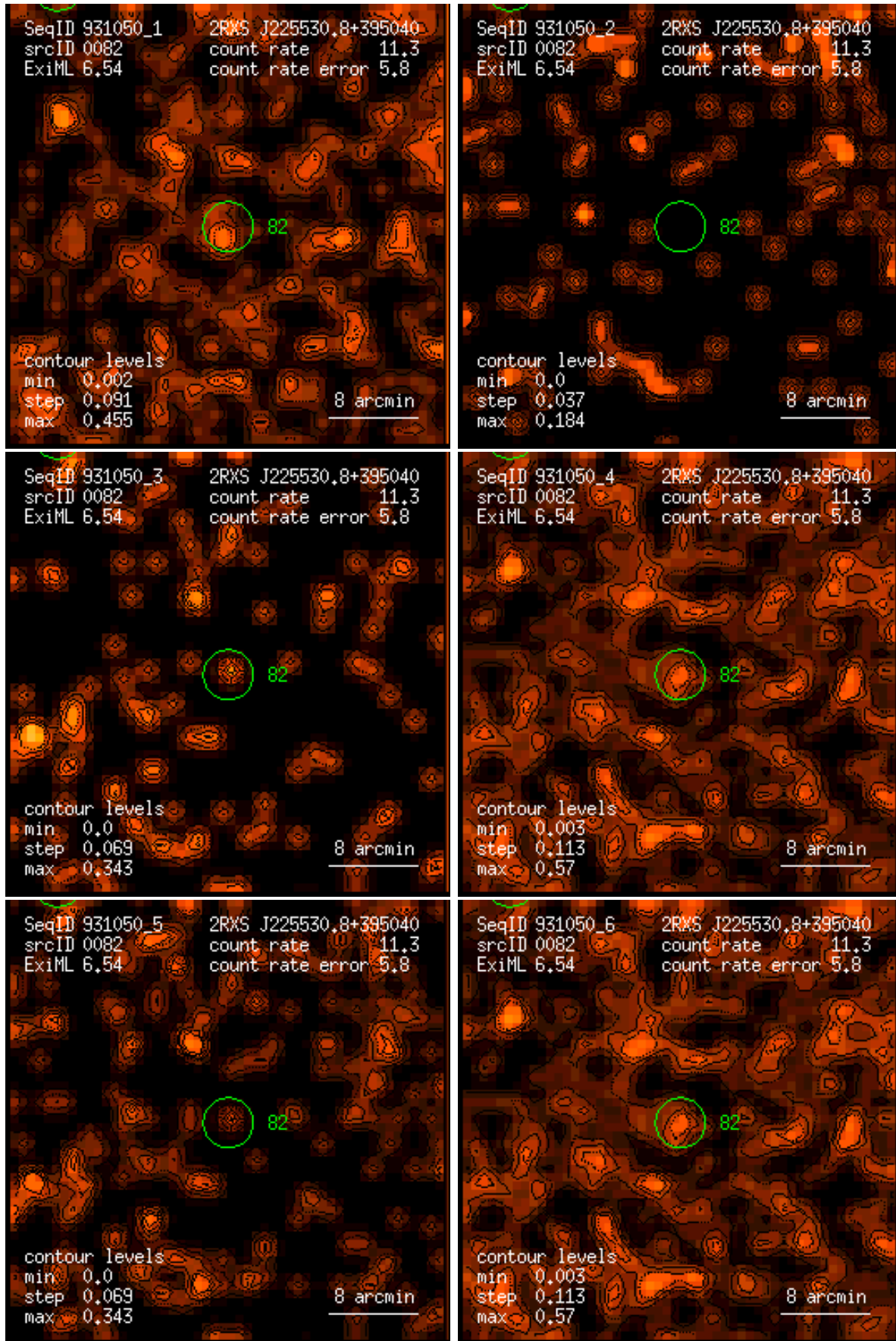
Figure 82: RASS 931050: detection 0082: band rate images, Gaussian filter: (1) PSPC channels 11 – 41, (2) 52 – 90, (3) 91 – 201, (4) 11 – 235, (5) 52 – 201, (6) 11 – 201. Broad band rates in counts/ks. Band rate contour levels in counts/ks/arcmin 2 .
