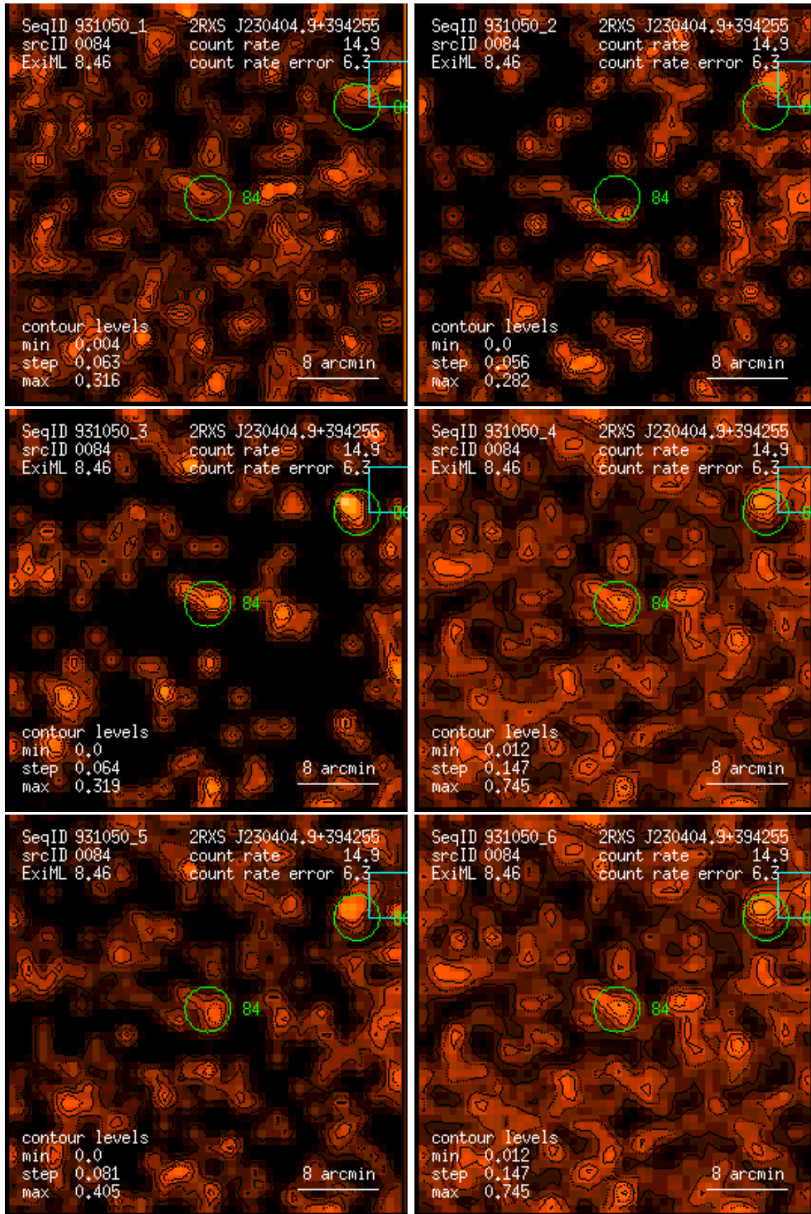
Figure 84: RASS 931050: detection 0084: band rate images, Gaussian filter: (1) PSPC channels 11 – 41, (2) 52 – 90, (3) 91 – 201, (4) 11 – 235, (5) 52 – 201, (6) 11 – 201. Broad band rates in counts/ks. Band rate contour levels in counts/ks/arcmin 2 .
