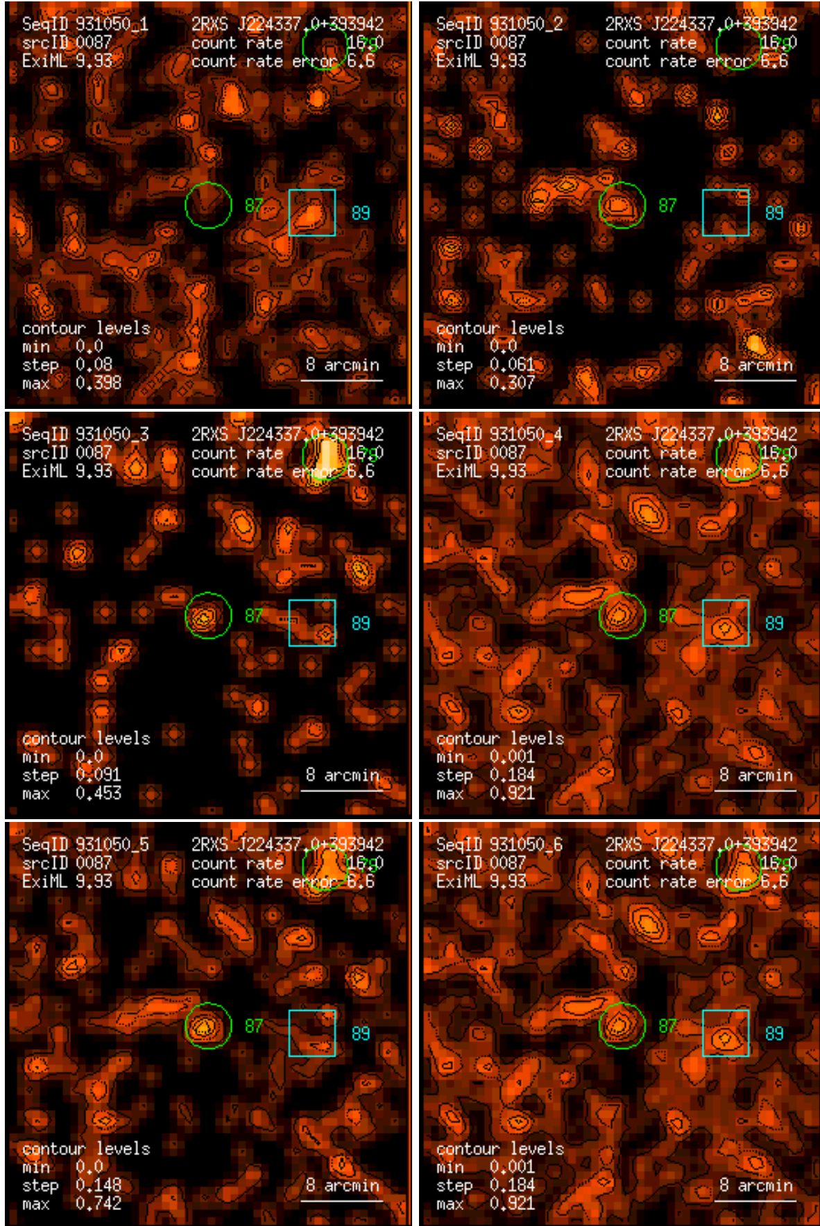
Figure 87: RASS 931050: detection 0087: band rate images, Gaussian filter: (1) PSPC channels 11 – 41, (2) 52 – 90, (3) 91 – 201, (4) 11 – 235, (5) 52 – 201, (6) 11 – 201. Broad band rates in counts/ks. Band rate contour levels in counts/ks/arcmin 2 .
