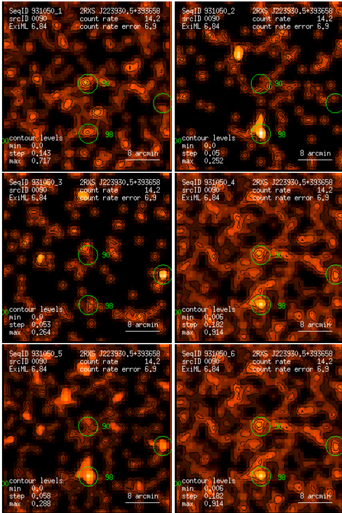
Figure 90: RASS 931050: detection 0090: band rate images, Gaussian filter: (1) PSPC channels 11 – 41, (2) 52 – 90, (3) 91 – 201, (4) 11 – 235, (5) 52 – 201, (6) 11 – 201. Broad band rates in counts/ks. Band rate contour levels in counts/ks/arcmin 2 .
