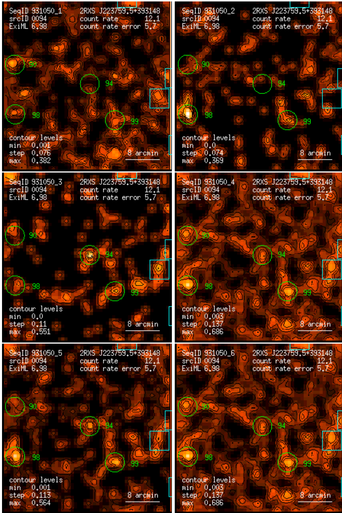
Figure 94: RASS 931050: detection 0094: band rate images, Gaussian filter: (1) PSPC channels 11 – 41, (2) 52 – 90, (3) 91 – 201, (4) 11 – 235, (5) 52 – 201, (6) 11 – 201. Broad band rates in counts/ks. Band rate contour levels in counts/ks/arcmin 2 .
