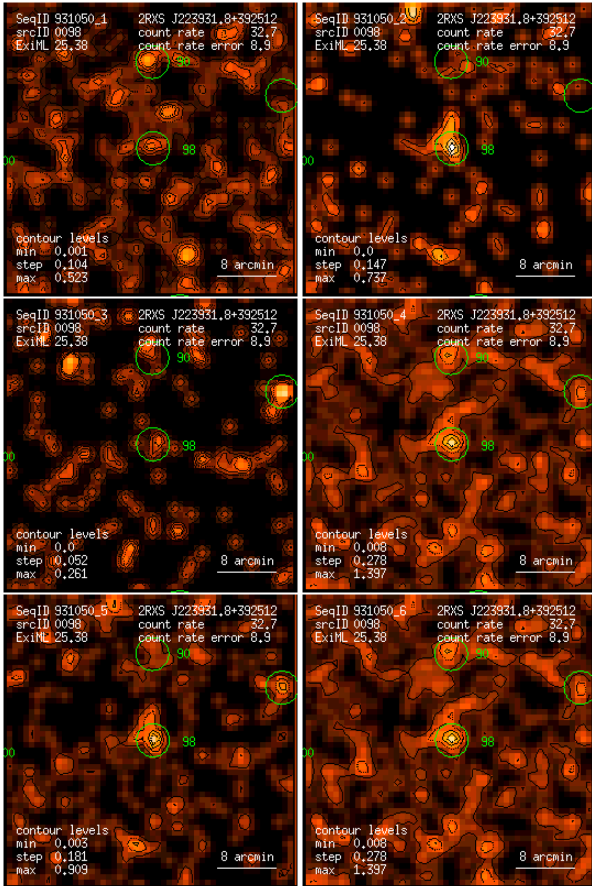
Figure 98: RASS 931050: detection 0098: band rate images, Gaussian filter: (1) PSPC channels 11 – 41, (2) 52 – 90, (3) 91 – 201, (4) 11 – 235, (5) 52 – 201, (6) 11 – 201. Broad band rates in counts/ks. Band rate contour levels in counts/ks/arcmin 2 .
