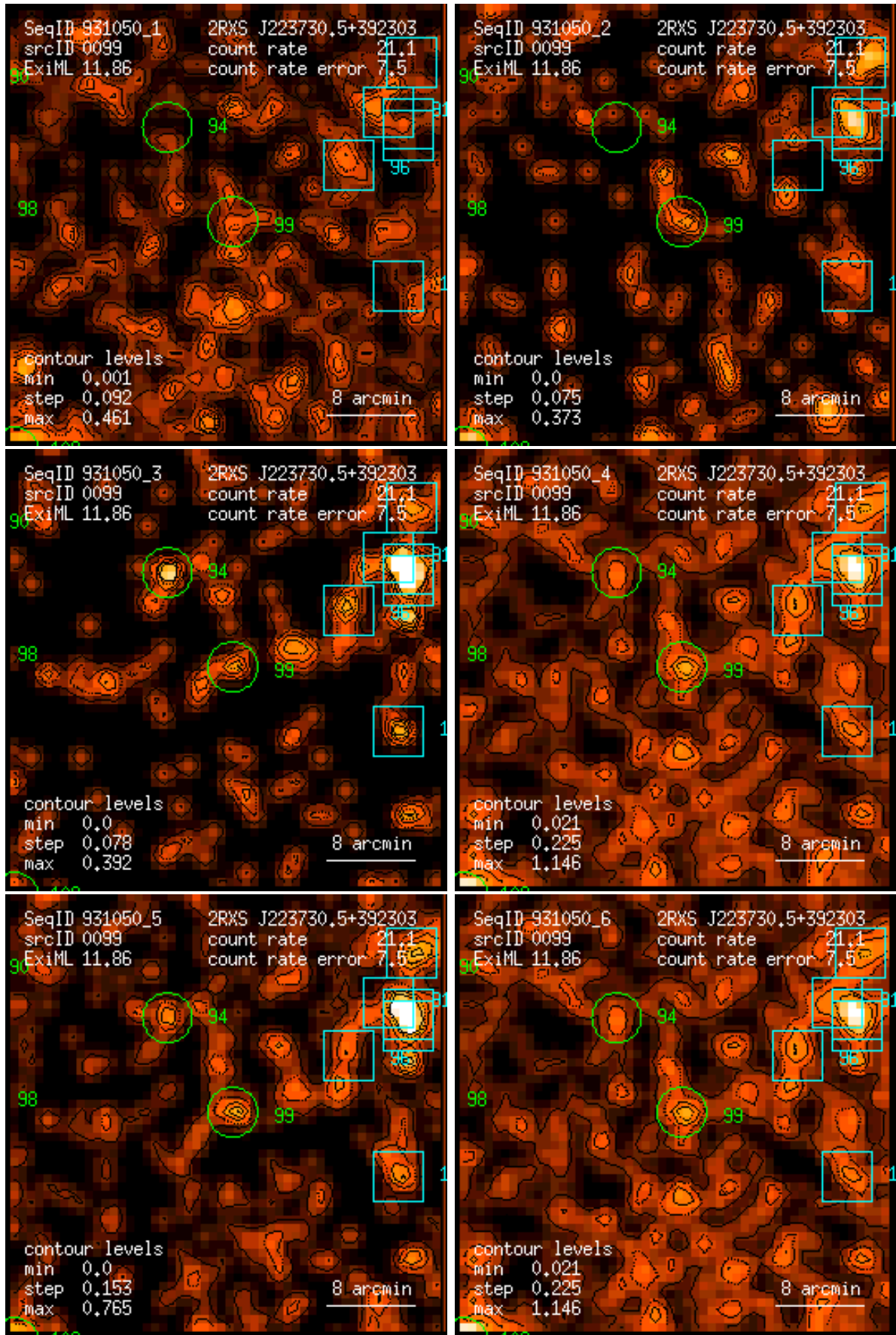
Figure 99: RASS 931050: detection 0099: band rate images, Gaussian filter: (1) PSPC channels 11 – 41, (2) 52 – 90, (3) 91 – 201, (4) 11 – 235, (5) 52 – 201, (6) 11 – 201. Broad band rates in counts/ks. Band rate contour levels in counts/ks/arcmin 2 .
