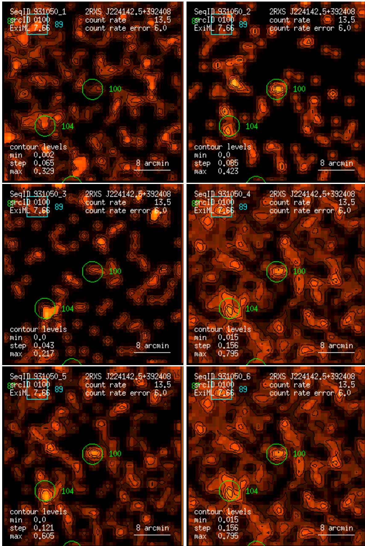
Figure 100: RASS 931050: detection 0100: band rate images, Gaussian filter: (1) PSPC channels 11 – 41, (2) 52 – 90, (3) 91 – 201, (4) 11 – 235, (5) 52 – 201, (6) 11 – 201. Broad band rates in counts/ks. Band rate contour levels in counts/ks/arcmin 2 .
