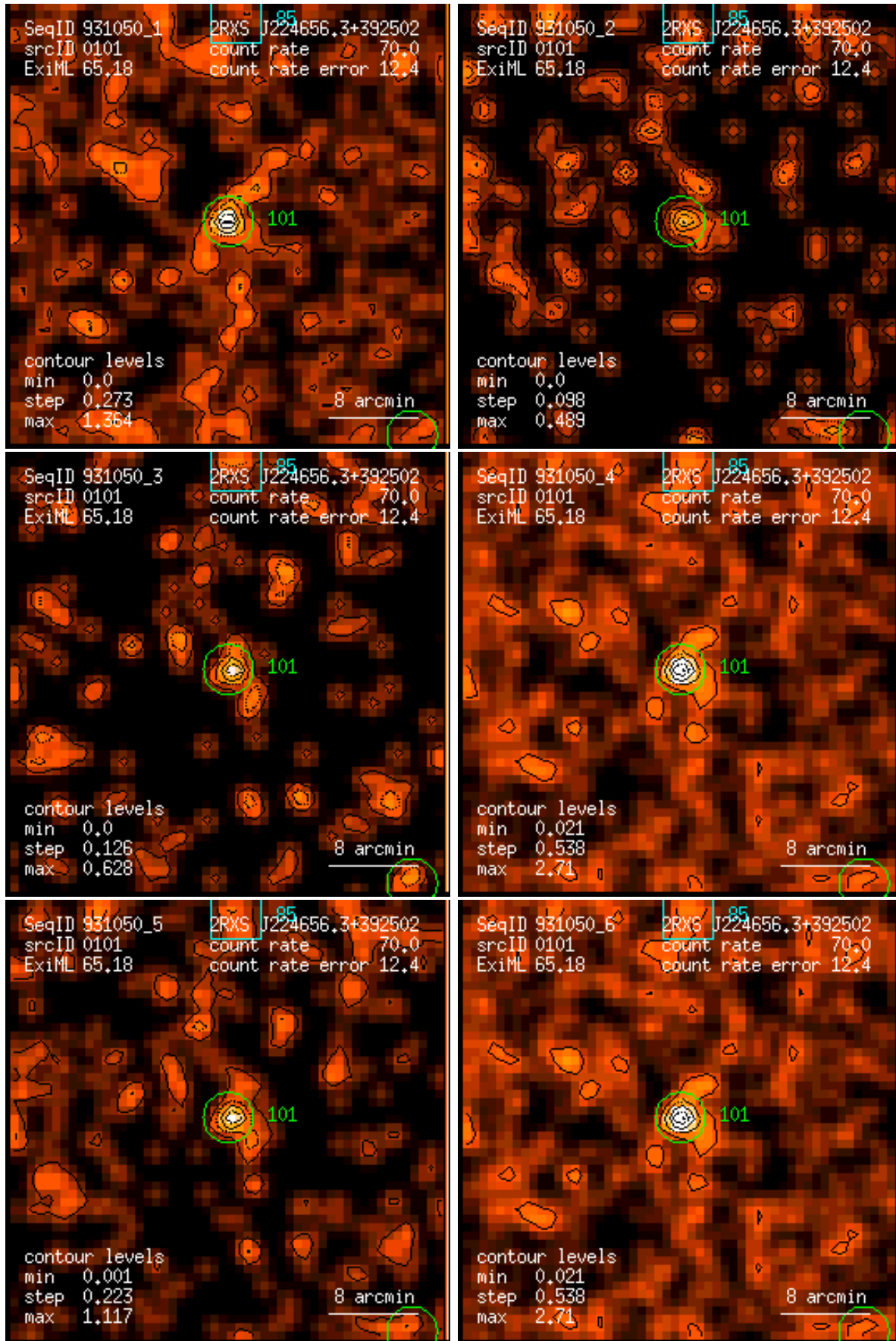
Figure 101: RASS 931050: detection 0101: band rate images, Gaussian filter: (1) PSPC channels 11 – 41, (2) 52 – 90, (3) 91 – 201, (4) 11 – 235, (5) 52 – 201, (6) 11 – 201. Broad band rates in counts/ks. Band rate contour levels in counts/ks/arcmin 2 .
