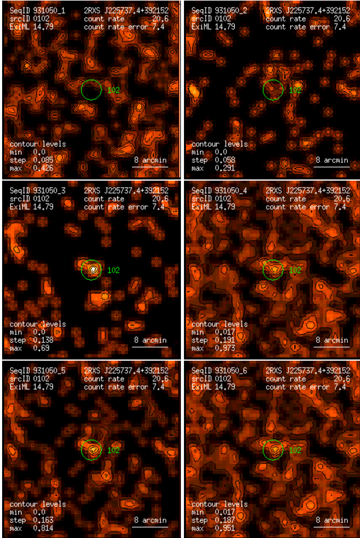
Figure 102: RASS 931050: detection 0102: band rate images, Gaussian filter: (1) PSPC channels 11 – 41, (2) 52 – 90, (3) 91 – 201, (4) 11 – 235, (5) 52 – 201, (6) 11 – 201. Broad band rates in counts/ks. Band rate contour levels in counts/ks/arcmin 2 .
