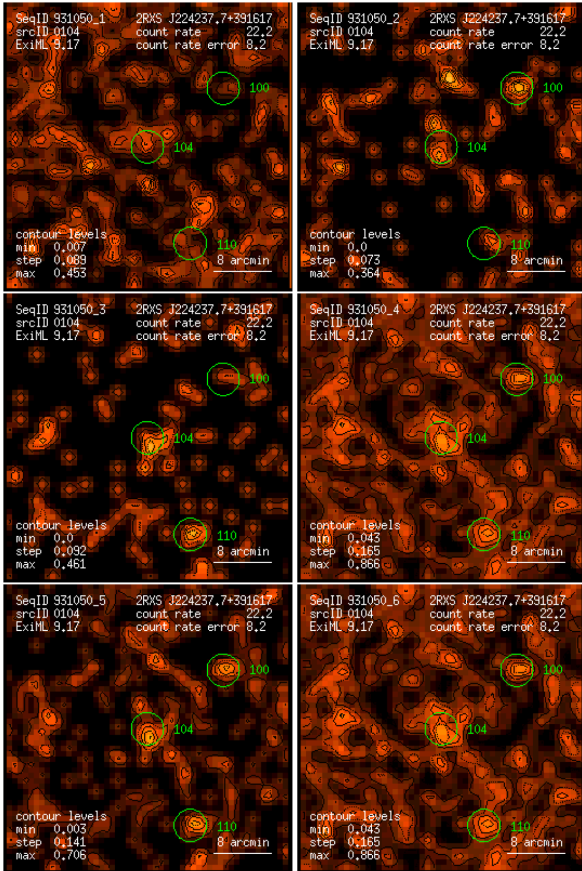
Figure 104: RASS 931050: detection 0104: band rate images, Gaussian filter: (1) PSPC channels 11 – 41, (2) 52 – 90, (3) 91 – 201, (4) 11 – 235, (5) 52 – 201, (6) 11 – 201. Broad band rates in counts/ks. Band rate contour levels in counts/ks/arcmin 2 .
