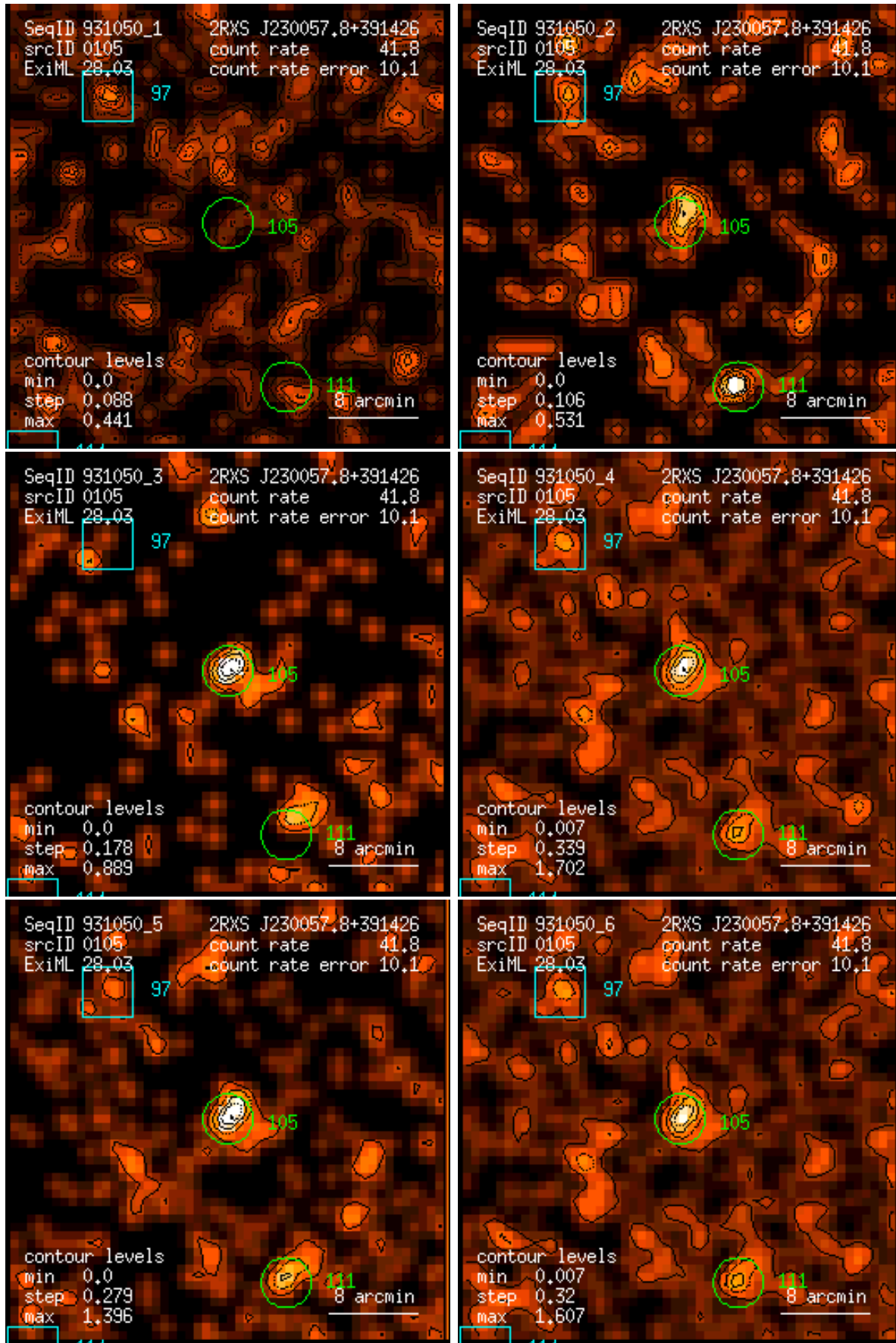
Figure 105: RASS 931050: detection 0105: band rate images, Gaussian filter: (1) PSPC channels 11 – 41, (2) 52 – 90, (3) 91 – 201, (4) 11 – 235, (5) 52 – 201, (6) 11 – 201. Broad band rates in counts/ks. Band rate contour levels in counts/ks/arcmin 2 .
