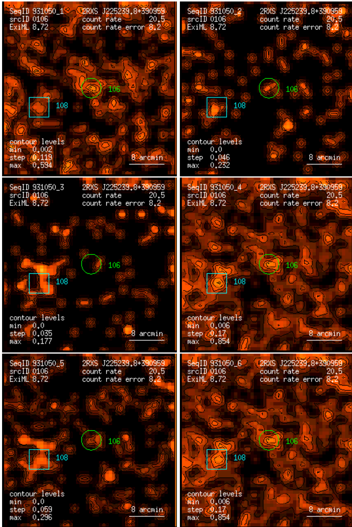
Figure 106: RASS 931050: detection 0106: band rate images, Gaussian filter: (1) PSPC channels 11 – 41, (2) 52 – 90, (3) 91 – 201, (4) 11 – 235, (5) 52 – 201, (6) 11 – 201. Broad band rates in counts/ks. Band rate contour levels in counts/ks/arcmin 2 .
