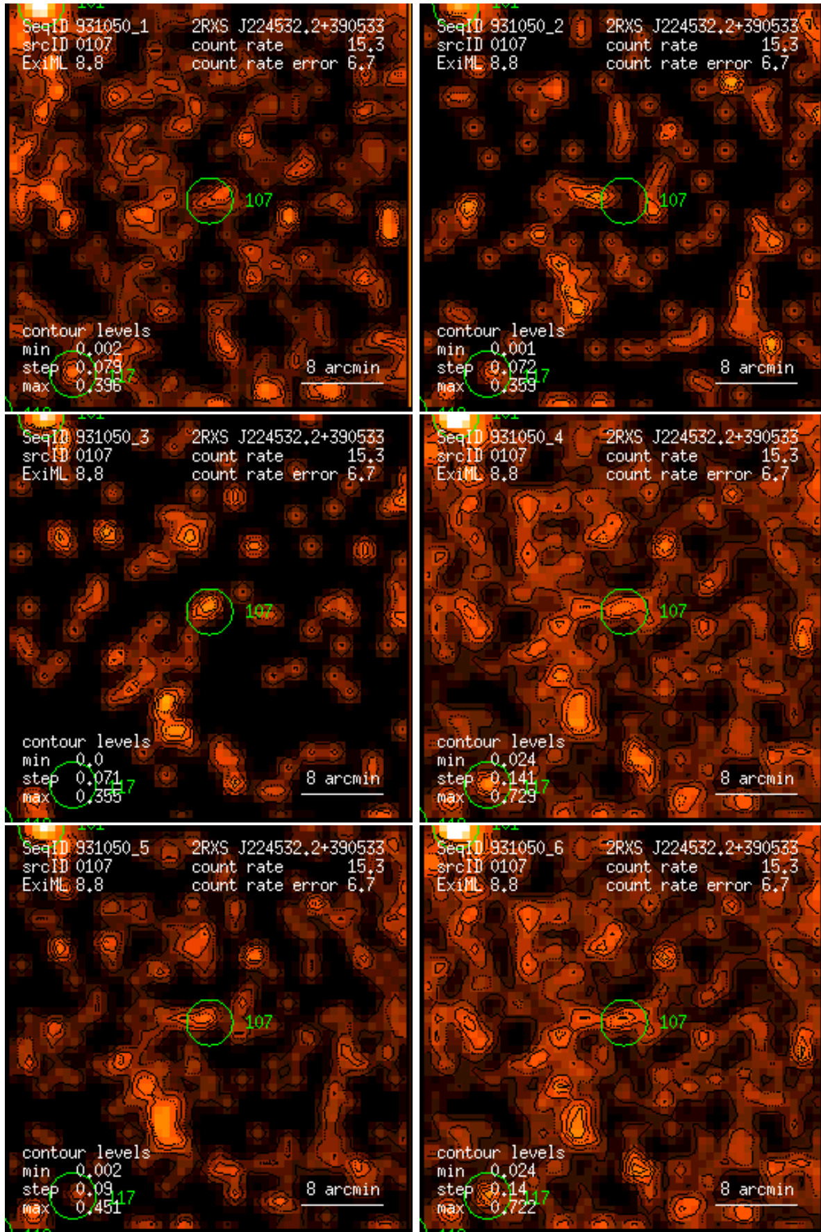
Figure 107: RASS 931050: detection 0107: band rate images, Gaussian filter: (1) PSPC channels 11 – 41, (2) 52 – 90, (3) 91 – 201, (4) 11 – 235, (5) 52 – 201, (6) 11 – 201. Broad band rates in counts/ks. Band rate contour levels in counts/ks/arcmin 2 .
