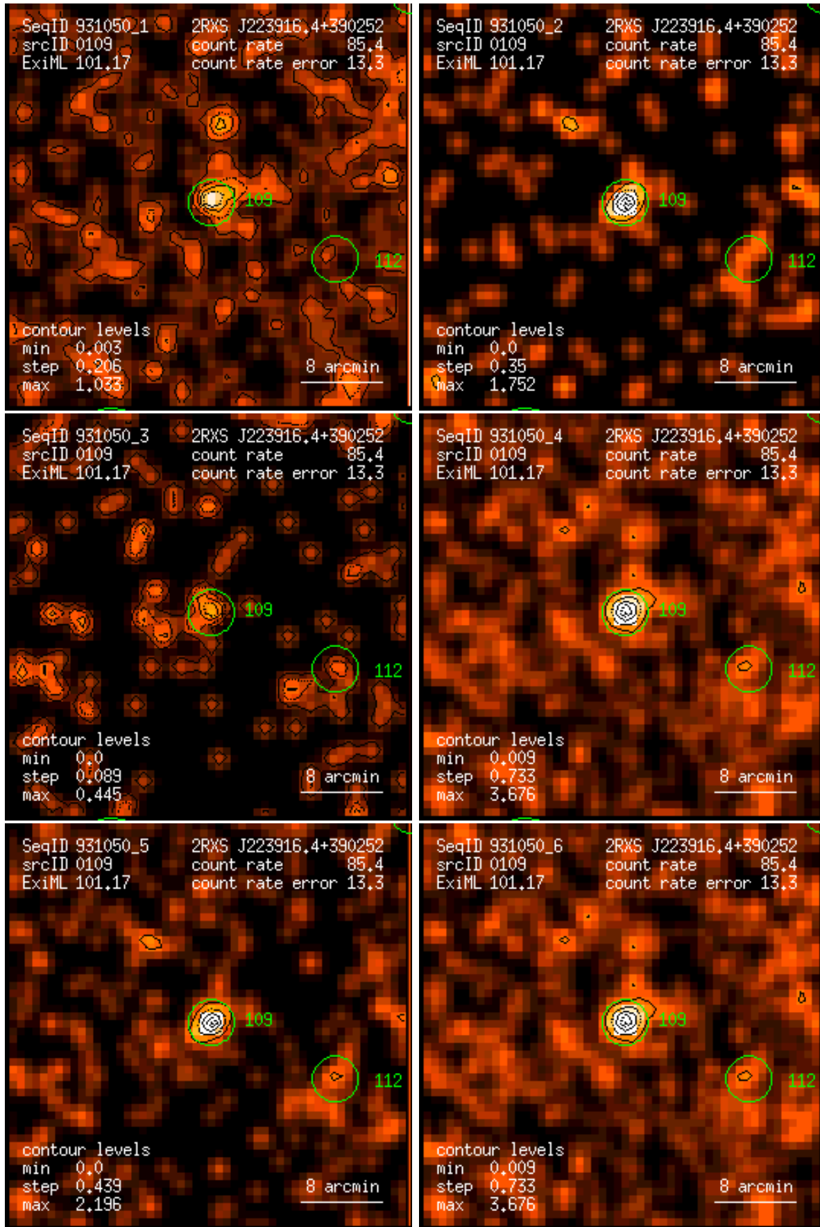
Figure 109: RASS 931050: detection 0109: band rate images, Gaussian filter: (1) PSPC channels 11 – 41, (2) 52 – 90, (3) 91 – 201, (4) 11 – 235, (5) 52 – 201, (6) 11 – 201. Broad band rates in counts/ks. Band rate contour levels in counts/ks/arcmin 2 .
