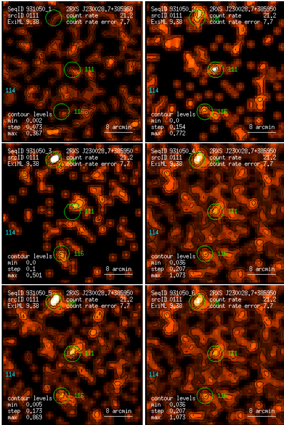
Figure 111: RASS 931050: detection 0111: band rate images, Gaussian filter: (1) PSPC channels 11 – 41, (2) 52 – 90, (3) 91 – 201, (4) 11 – 235, (5) 52 – 201, (6) 11 – 201. Broad band rates in counts/ks. Band rate contour levels in counts/ks/arcmin 2 .
