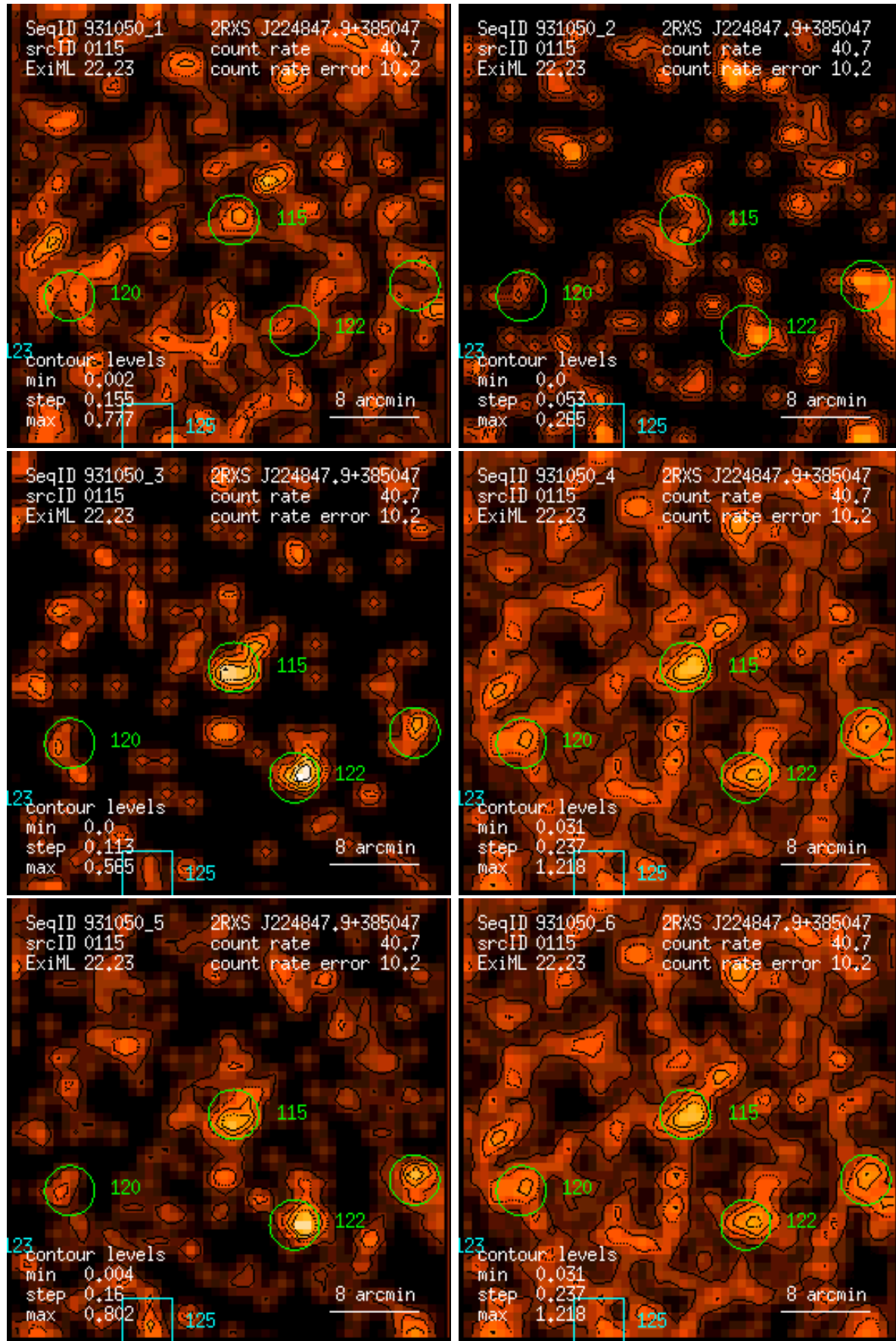
Figure 115: RASS 931050: detection 0115: band rate images, Gaussian filter: (1) PSPC channels 11 – 41, (2) 52 – 90, (3) 91 – 201, (4) 11 – 235, (5) 52 – 201, (6) 11 – 201. Broad band rates in counts/ks. Band rate contour levels in counts/ks/arcmin 2 .
