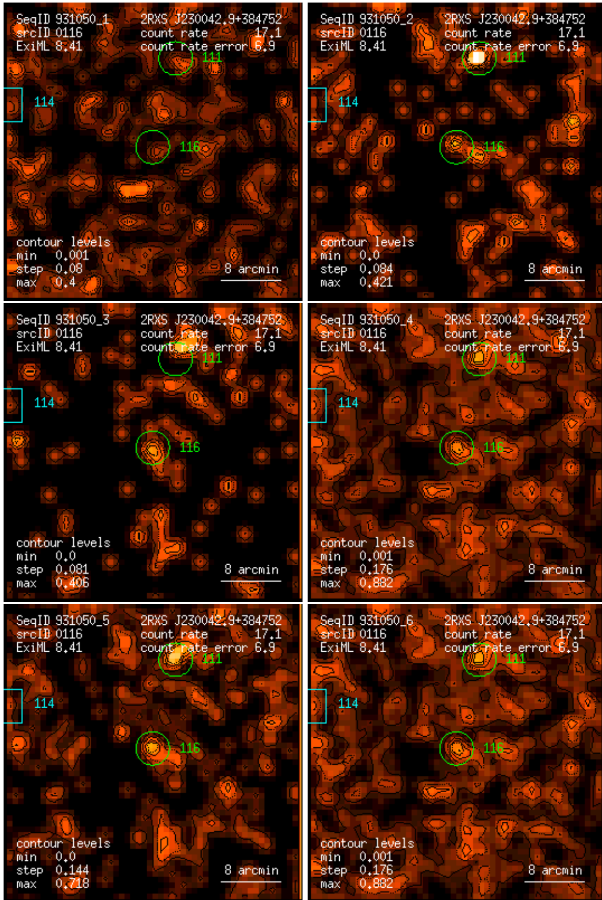
Figure 116: RASS 931050: detection 0116: band rate images, Gaussian filter: (1) PSPC channels 11 – 41, (2) 52 – 90, (3) 91 – 201, (4) 11 – 235, (5) 52 – 201, (6) 11 – 201. Broad band rates in counts/ks. Band rate contour levels in counts/ks/arcmin 2 .
