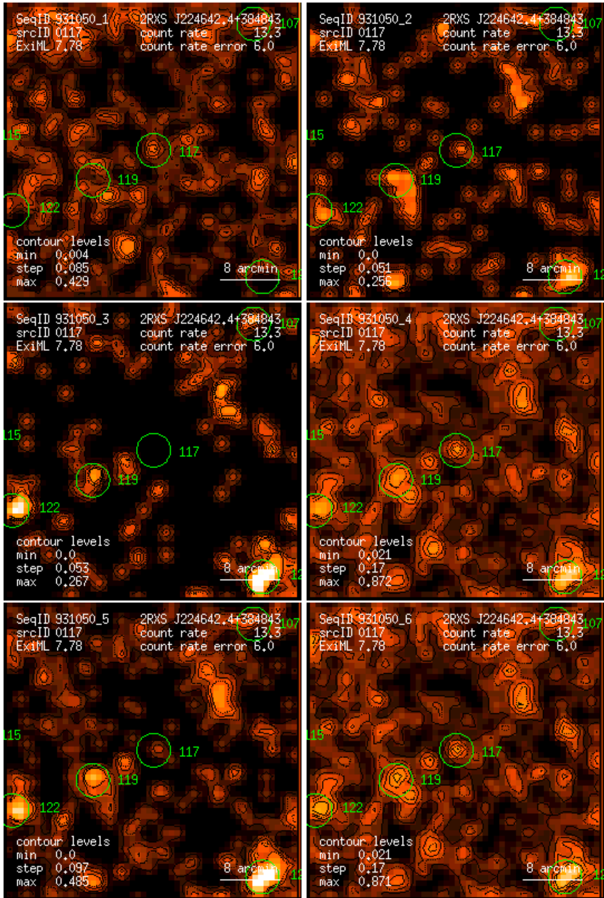
Figure 117: RASS 931050: detection 0117: band rate images, Gaussian filter: (1) PSPC channels 11 – 41, (2) 52 – 90, (3) 91 – 201, (4) 11 – 235, (5) 52 – 201, (6) 11 – 201. Broad band rates in counts/ks. Band rate contour levels in counts/ks/arcmin 2 .
