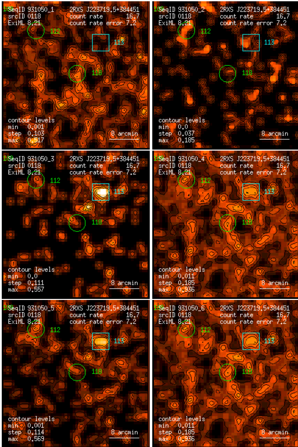
Figure 118: RASS 931050: detection 0118: band rate images, Gaussian filter: (1) PSPC channels 11 – 41, (2) 52 – 90, (3) 91 – 201, (4) 11 – 235, (5) 52 – 201, (6) 11 – 201. Broad band rates in counts/ks. Band rate contour levels in counts/ks/arcmin 2 .
