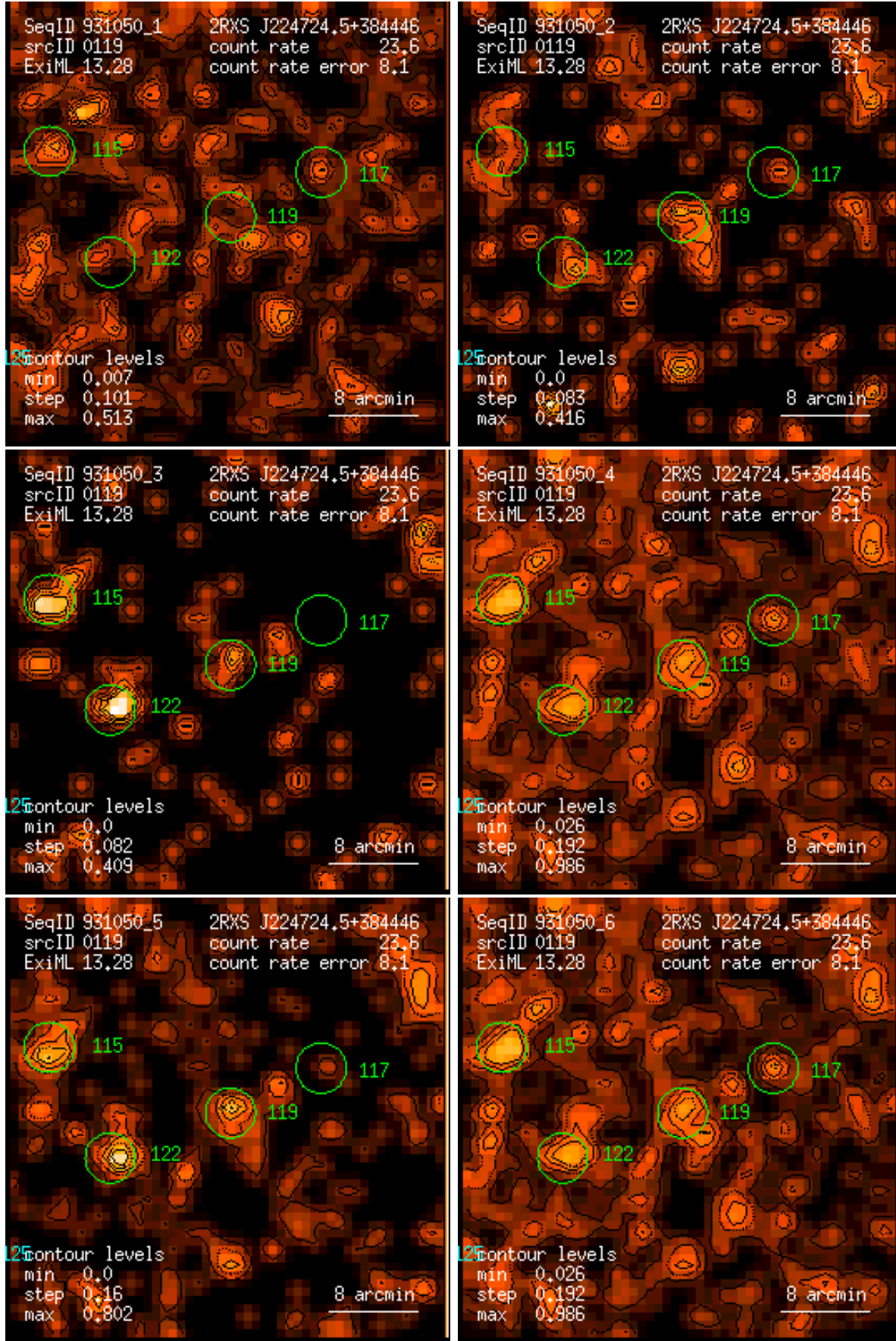
Figure 119: RASS 931050: detection 0119: band rate images, Gaussian filter: (1) PSPC channels 11 – 41, (2) 52 – 90, (3) 91 – 201, (4) 11 – 235, (5) 52 – 201, (6) 11 – 201. Broad band rates in counts/ks. Band rate contour levels in counts/ks/arcmin 2 .
