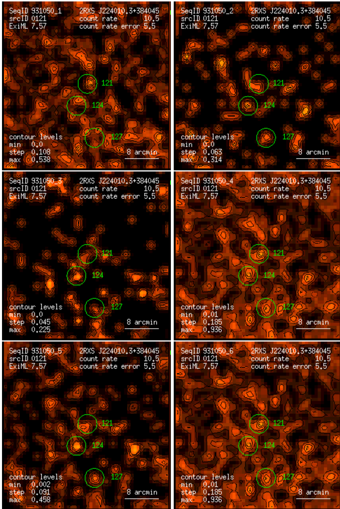
Figure 121: RASS 931050: detection 0121: band rate images, Gaussian filter: (1) PSPC channels 11 – 41, (2) 52 – 90, (3) 91 – 201, (4) 11 – 235, (5) 52 – 201, (6) 11 – 201. Broad band rates in counts/ks. Band rate contour levels in counts/ks/arcmin 2 .
