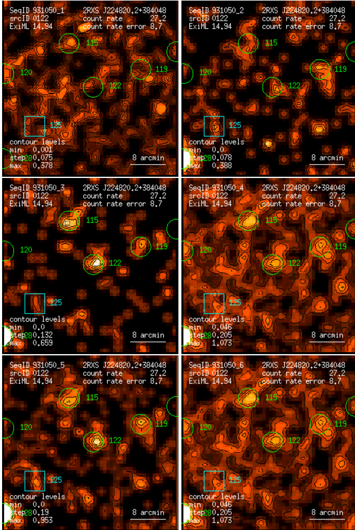
Figure 122: RASS 931050: detection 0122: band rate images, Gaussian filter: (1) PSPC channels 11 – 41, (2) 52 – 90, (3) 91 – 201, (4) 11 – 235, (5) 52 – 201, (6) 11 – 201. Broad band rates in counts/ks. Band rate contour levels in counts/ks/arcmin 2 .
