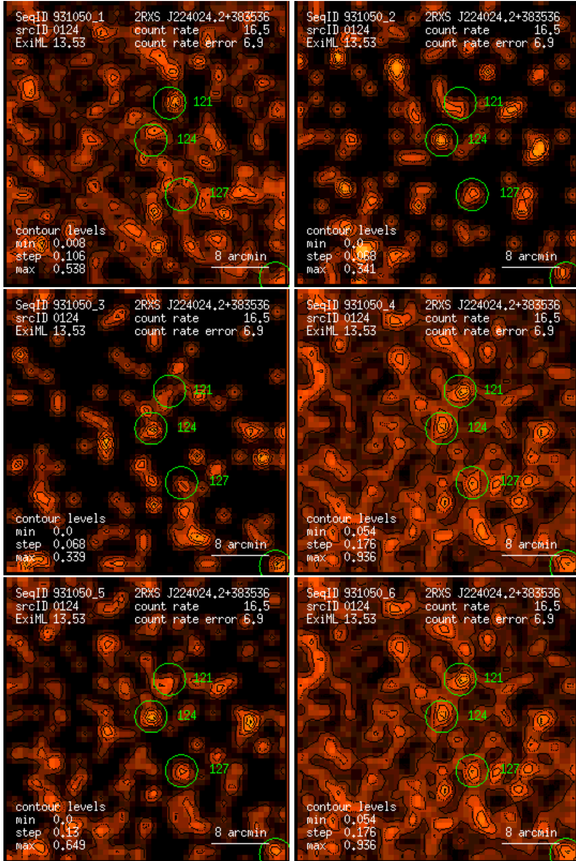
Figure 124: RASS 931050: detection 0124: band rate images, Gaussian filter: (1) PSPC channels 11 – 41, (2) 52 – 90, (3) 91 – 201, (4) 11 – 235, (5) 52 – 201, (6) 11 – 201. Broad band rates in counts/ks. Band rate contour levels in counts/ks/arcmin 2 .
