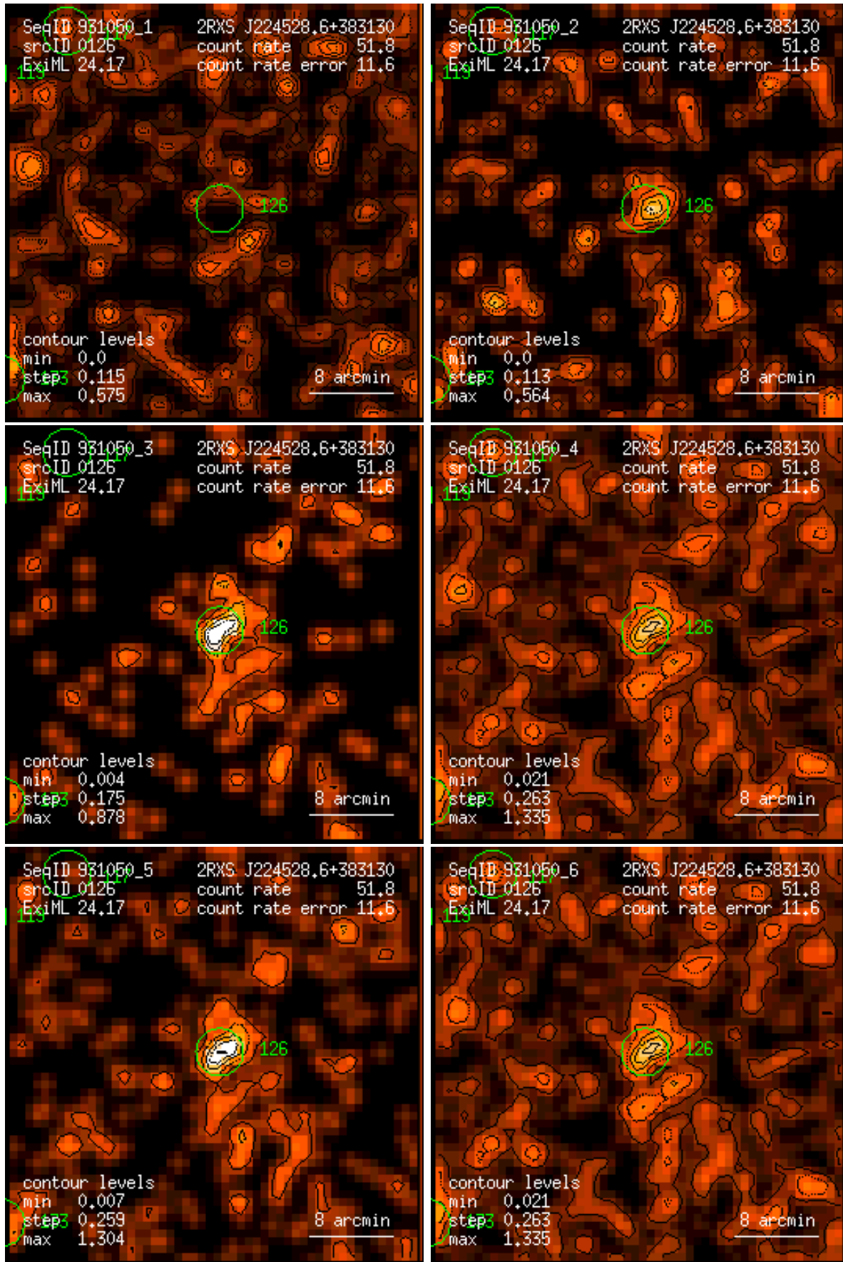
Figure 126: RASS 931050: detection 0126: band rate images, Gaussian filter: (1) PSPC channels 11 – 41, (2) 52 – 90, (3) 91 – 201, (4) 11 – 235, (5) 52 – 201, (6) 11 – 201. Broad band rates in counts/ks. Band rate contour levels in counts/ks/arcmin 2 .
