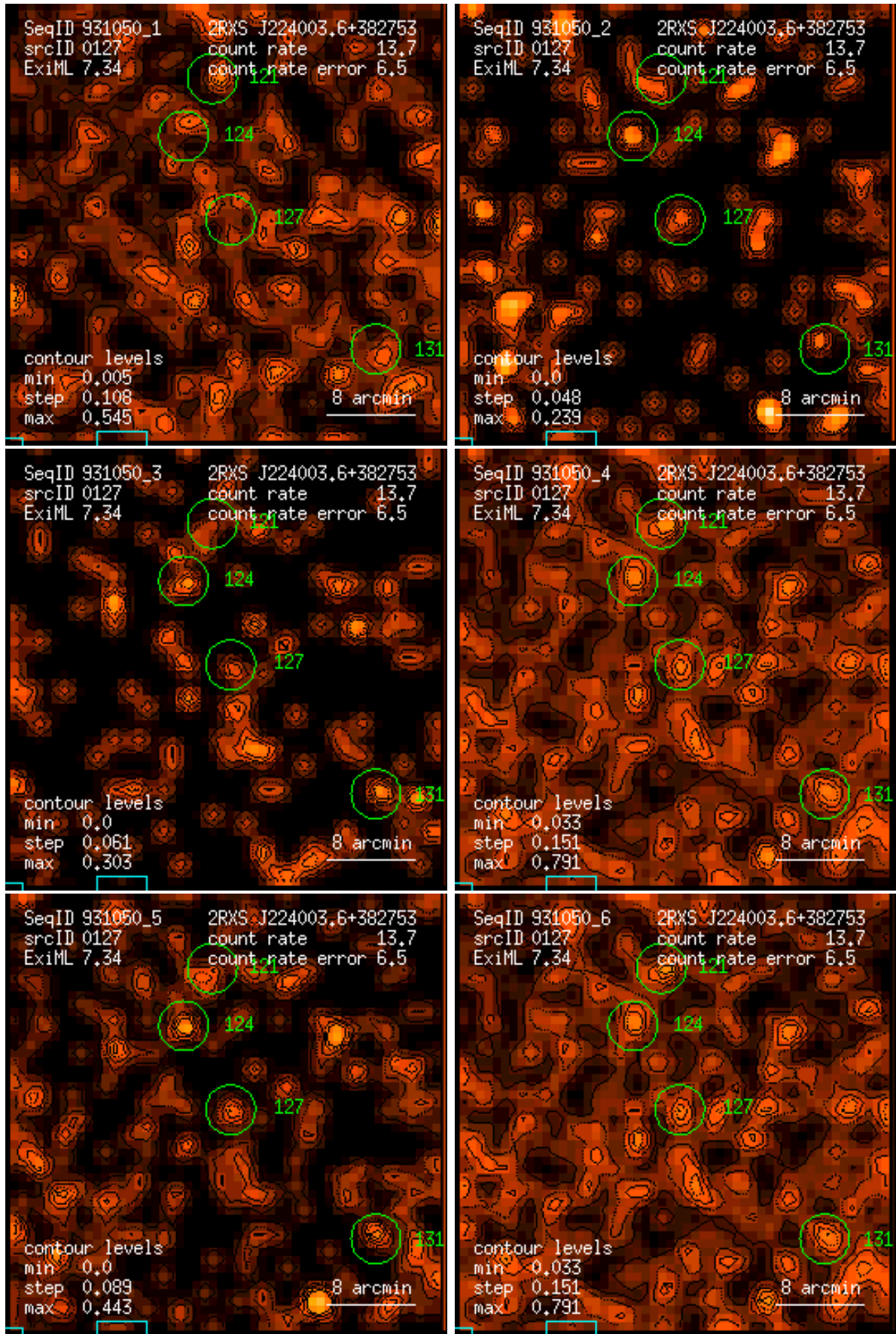
Figure 127: RASS 931050: detection 0127: band rate images, Gaussian filter: (1) PSPC channels 11 – 41, (2) 52 – 90, (3) 91 – 201, (4) 11 – 235, (5) 52 – 201, (6) 11 – 201. Broad band rates in counts/ks. Band rate contour levels in counts/ks/arcmin 2 .
