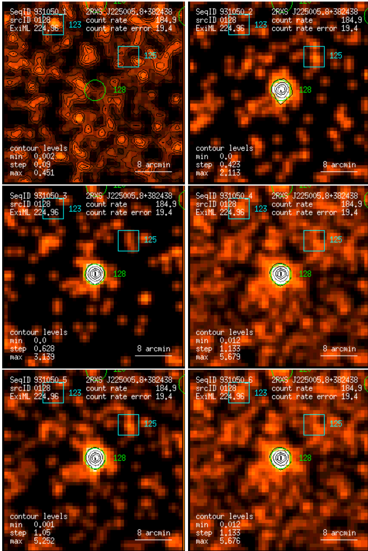
Figure 128: RASS 931050: detection 0128: band rate images, Gaussian filter: (1) PSPC channels 11 – 41, (2) 52 – 90, (3) 91 – 201, (4) 11 – 235, (5) 52 – 201, (6) 11 – 201. Broad band rates in counts/ks. Band rate contour levels in counts/ks/arcmin 2 .
