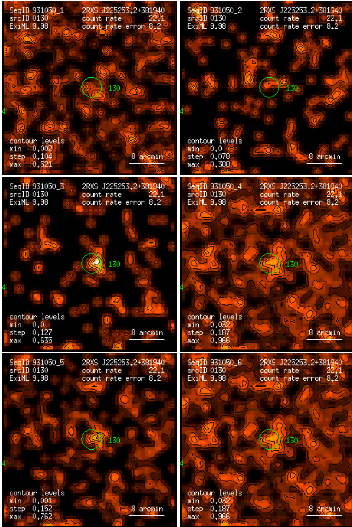
Figure 130: RASS 931050: detection 0130: band rate images, Gaussian filter: (1) PSPC channels 11 – 41, (2) 52 – 90, (3) 91 – 201, (4) 11 – 235, (5) 52 – 201, (6) 11 – 201. Broad band rates in counts/ks. Band rate contour levels in counts/ks/arcmin 2 .
