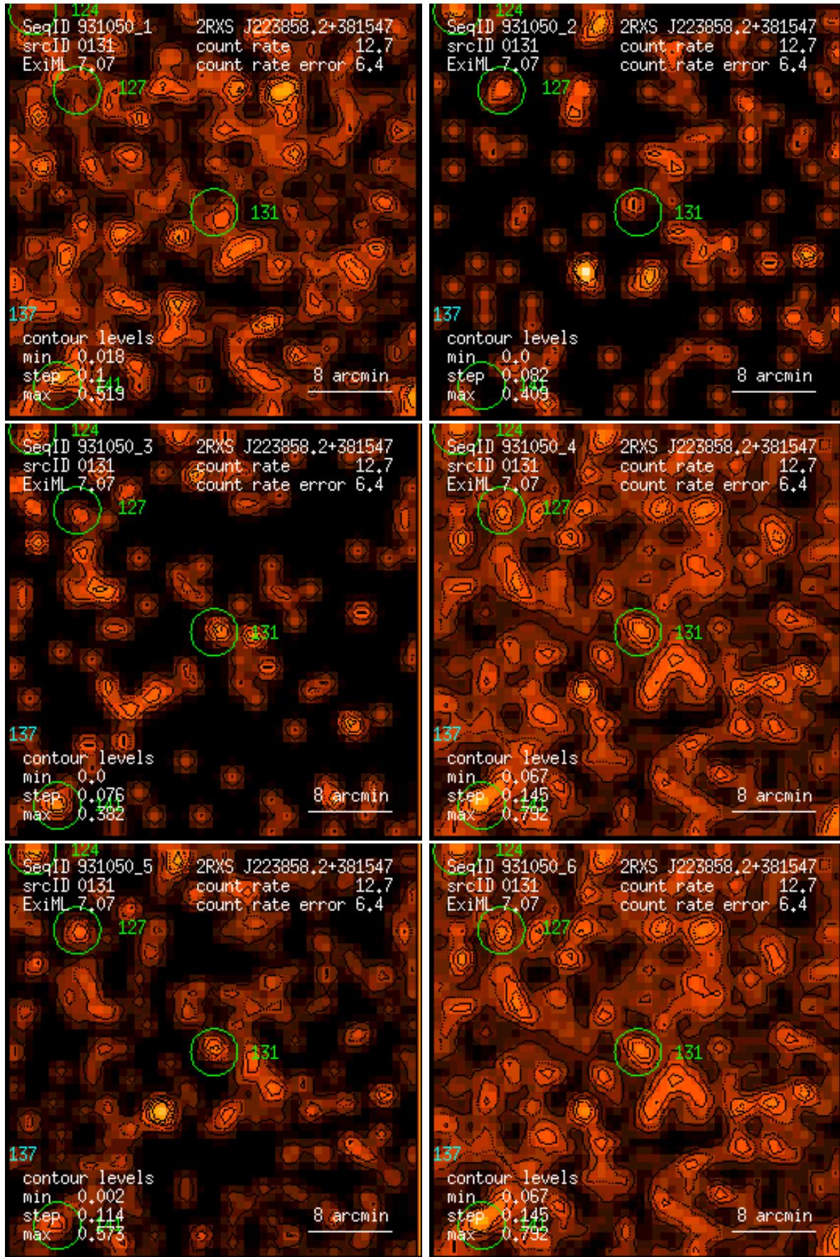
Figure 131: RASS 931050: detection 0131: band rate images, Gaussian filter: (1) PSPC channels 11 – 41, (2) 52 – 90, (3) 91 – 201, (4) 11 – 235, (5) 52 – 201, (6) 11 – 201. Broad band rates in counts/ks. Band rate contour levels in counts/ks/arcmin 2 .
