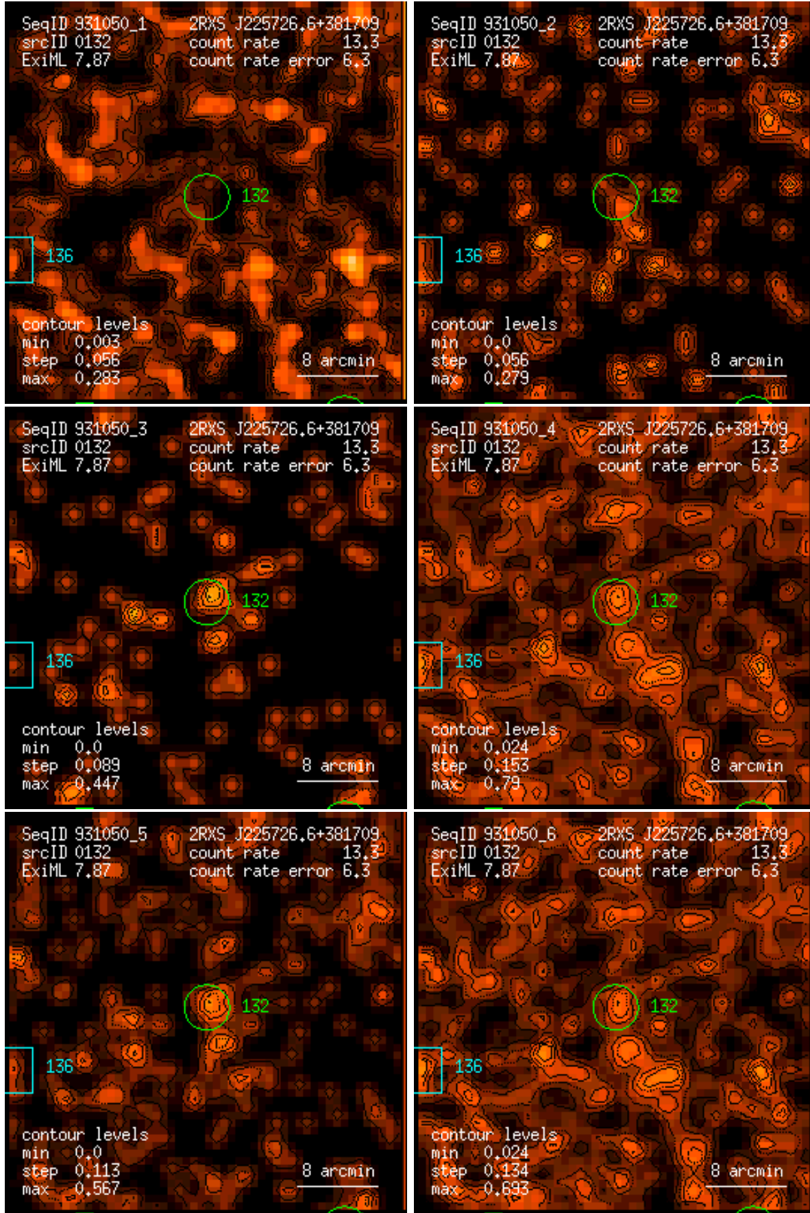
Figure 132: RASS 931050: detection 0132: band rate images, Gaussian filter: (1) PSPC channels 11 – 41, (2) 52 – 90, (3) 91 – 201, (4) 11 – 235, (5) 52 – 201, (6) 11 – 201. Broad band rates in counts/ks. Band rate contour levels in counts/ks/arcmin 2 .
