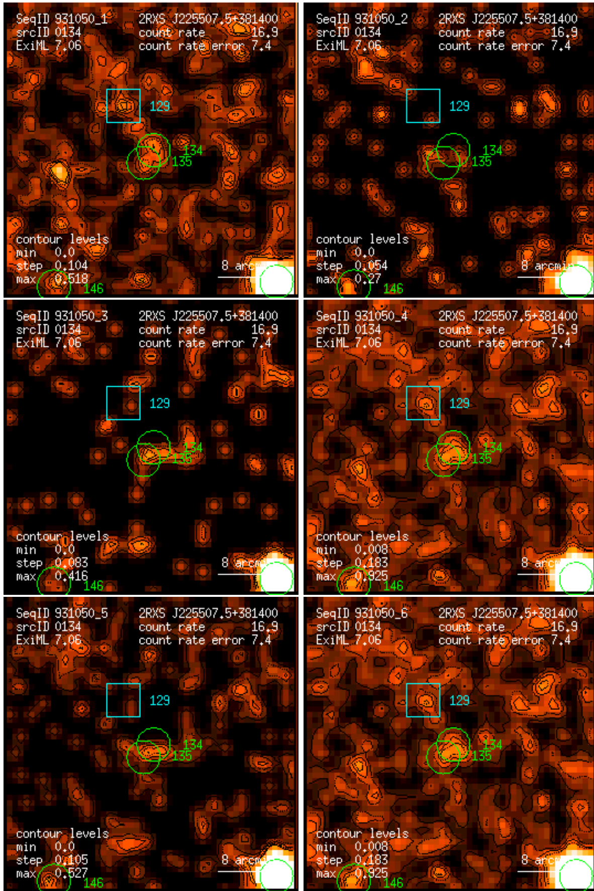
Figure 134: RASS 931050: detection 0134: band rate images, Gaussian filter: (1) PSPC channels 11 – 41, (2) 52 – 90, (3) 91 – 201, (4) 11 – 235, (5) 52 – 201, (6) 11 – 201. Broad band rates in counts/ks. Band rate contour levels in counts/ks/arcmin 2 .
