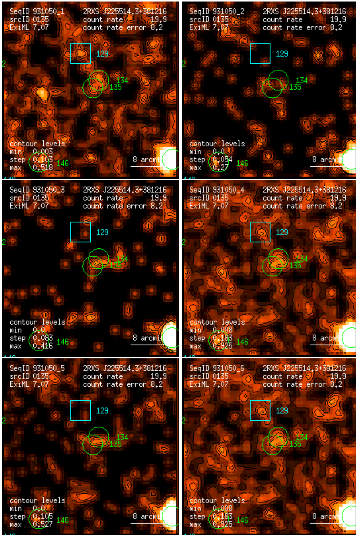
Figure 135: RASS 931050: detection 0135: band rate images, Gaussian filter: (1) PSPC channels 11 – 41, (2) 52 – 90, (3) 91 – 201, (4) 11 – 235, (5) 52 – 201, (6) 11 – 201. Broad band rates in counts/ks. Band rate contour levels in counts/ks/arcmin 2 .
