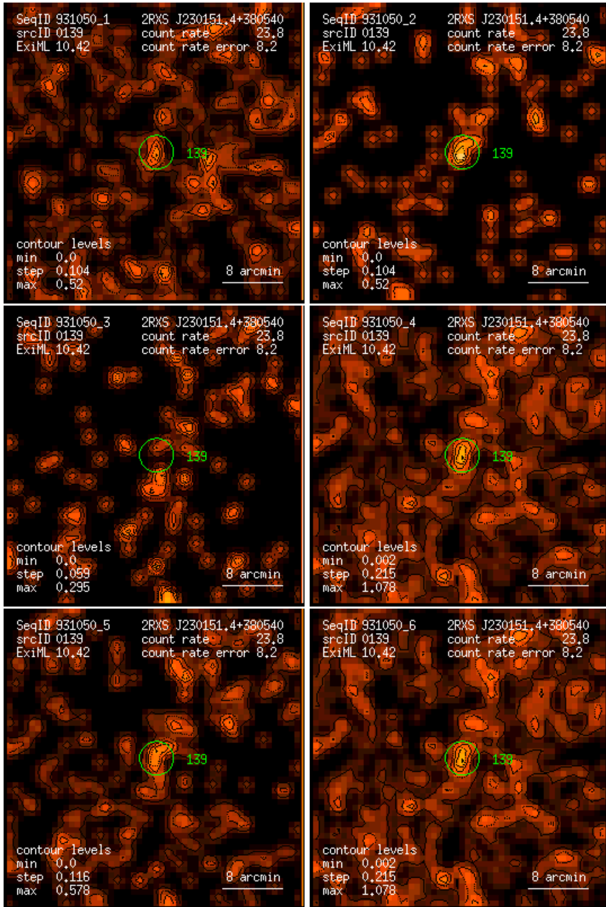
Figure 139: RASS 931050: detection 0139: band rate images, Gaussian filter: (1) PSPC channels 11 – 41, (2) 52 – 90, (3) 91 – 201, (4) 11 – 235, (5) 52 – 201, (6) 11 – 201. Broad band rates in counts/ks. Band rate contour levels in counts/ks/arcmin 2 .
