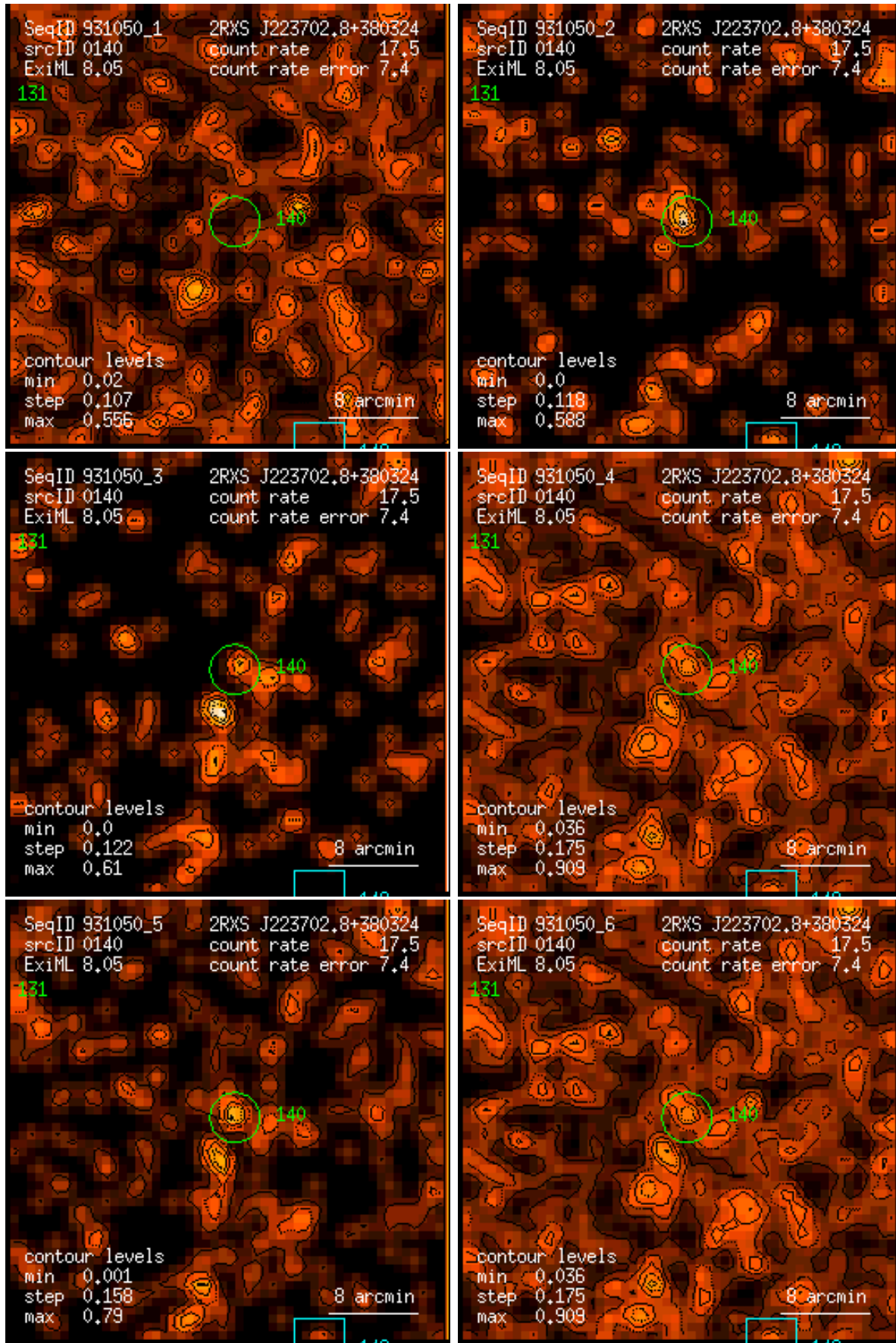
Figure 140: RASS 931050: detection 0140: band rate images, Gaussian filter: (1) PSPC channels 11 – 41, (2) 52 – 90, (3) 91 – 201, (4) 11 – 235, (5) 52 – 201, (6) 11 – 201. Broad band rates in counts/ks. Band rate contour levels in counts/ks/arcmin 2 .
