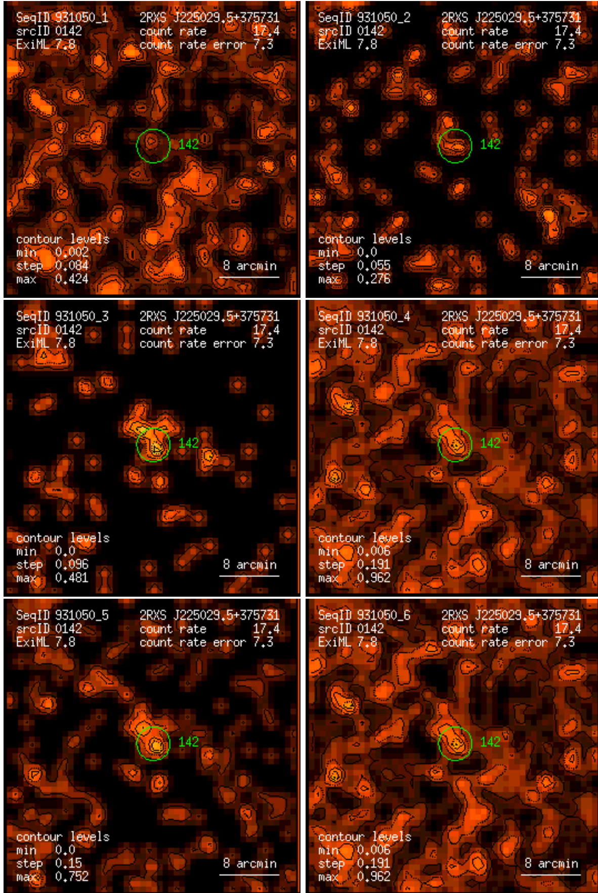
Figure 142: RASS 931050: detection 0142: band rate images, Gaussian filter: (1) PSPC channels 11 – 41, (2) 52 – 90, (3) 91 – 201, (4) 11 – 235, (5) 52 – 201, (6) 11 – 201. Broad band rates in counts/ks. Band rate contour levels in counts/ks/arcmin 2 .
