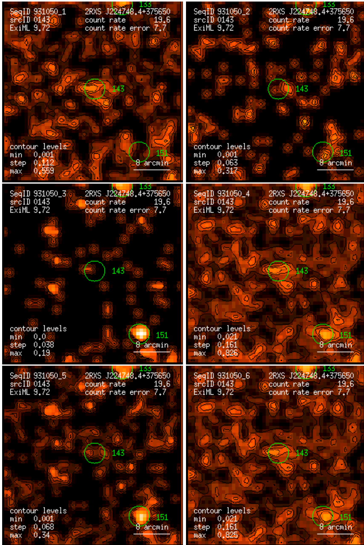
Figure 143: RASS 931050: detection 0143: band rate images, Gaussian filter: (1) PSPC channels 11 – 41, (2) 52 – 90, (3) 91 – 201, (4) 11 – 235, (5) 52 – 201, (6) 11 – 201. Broad band rates in counts/ks. Band rate contour levels in counts/ks/arcmin 2 .
