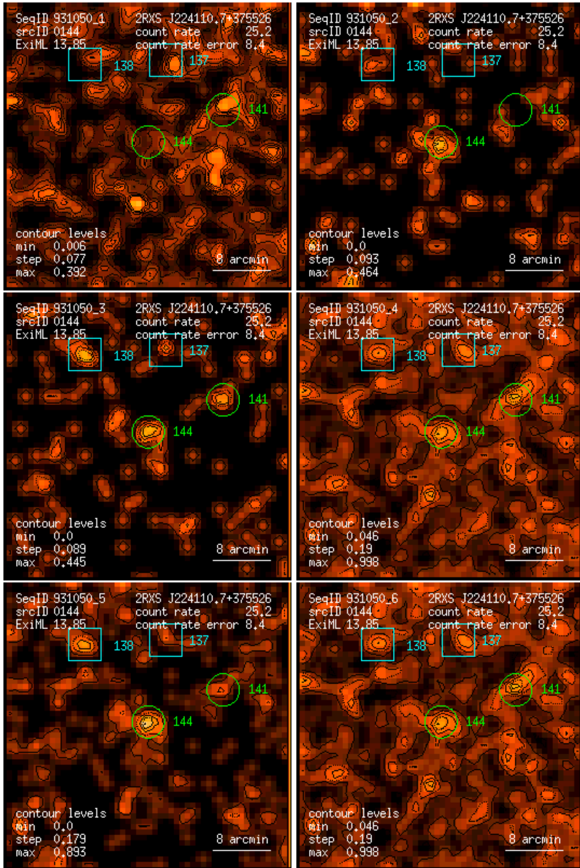
Figure 144: RASS 931050: detection 0144: band rate images, Gaussian filter: (1) PSPC channels 11 – 41, (2) 52 – 90, (3) 91 – 201, (4) 11 – 235, (5) 52 – 201, (6) 11 – 201. Broad band rates in counts/ks. Band rate contour levels in counts/ks/arcmin 2 .
