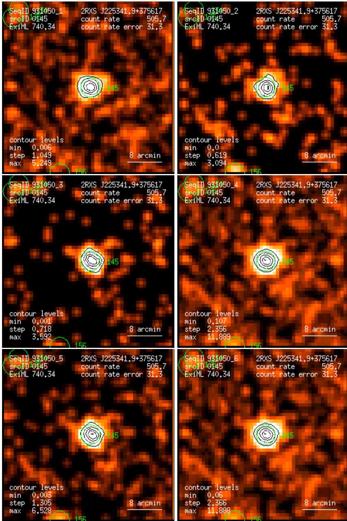
Figure 145: RASS 931050: detection 0145: band rate images, Gaussian filter: (1) PSPC channels 11 – 41, (2) 52 – 90, (3) 91 – 201, (4) 11 – 235, (5) 52 – 201, (6) 11 – 201. Broad band rates in counts/ks. Band rate contour levels in counts/ks/arcmin 2 .
