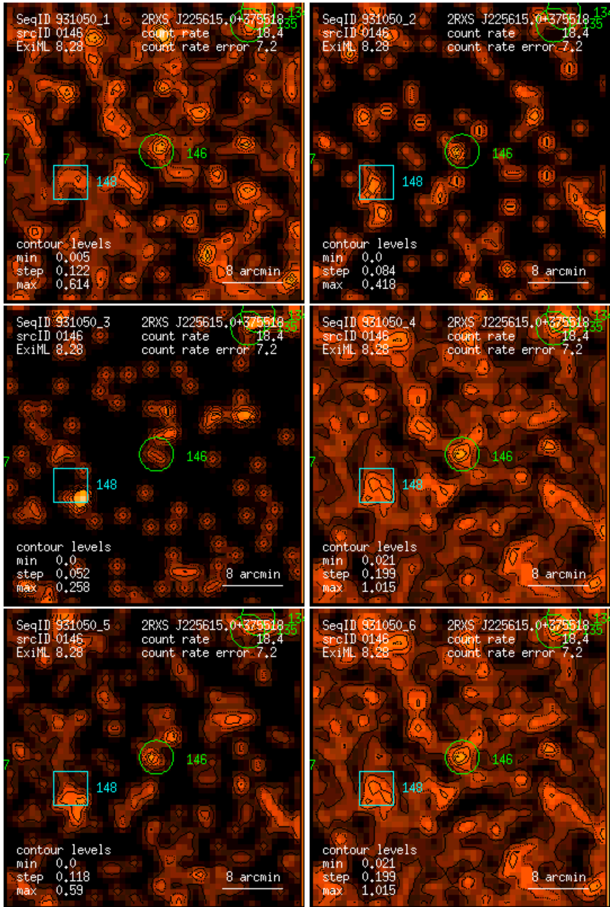
Figure 146: RASS 931050: detection 0146: band rate images, Gaussian filter: (1) PSPC channels 11 – 41, (2) 52 – 90, (3) 91 – 201, (4) 11 – 235, (5) 52 – 201, (6) 11 – 201. Broad band rates in counts/ks. Band rate contour levels in counts/ks/arcmin 2 .
