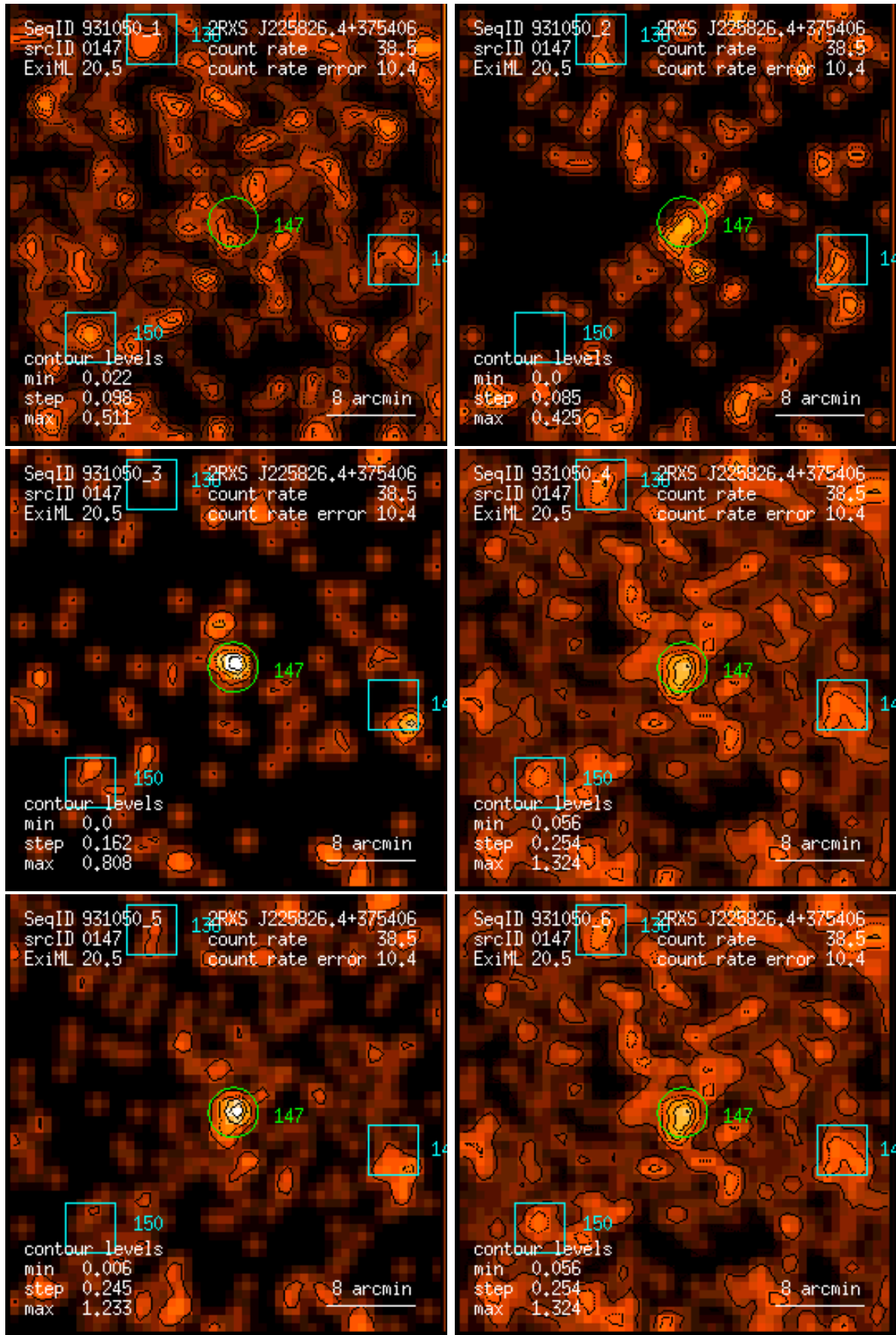
Figure 147: RASS 931050: detection 0147: band rate images, Gaussian filter: (1) PSPC channels 11 – 41, (2) 52 – 90, (3) 91 – 201, (4) 11 – 235, (5) 52 – 201, (6) 11 – 201. Broad band rates in counts/ks. Band rate contour levels in counts/ks/arcmin 2 .
