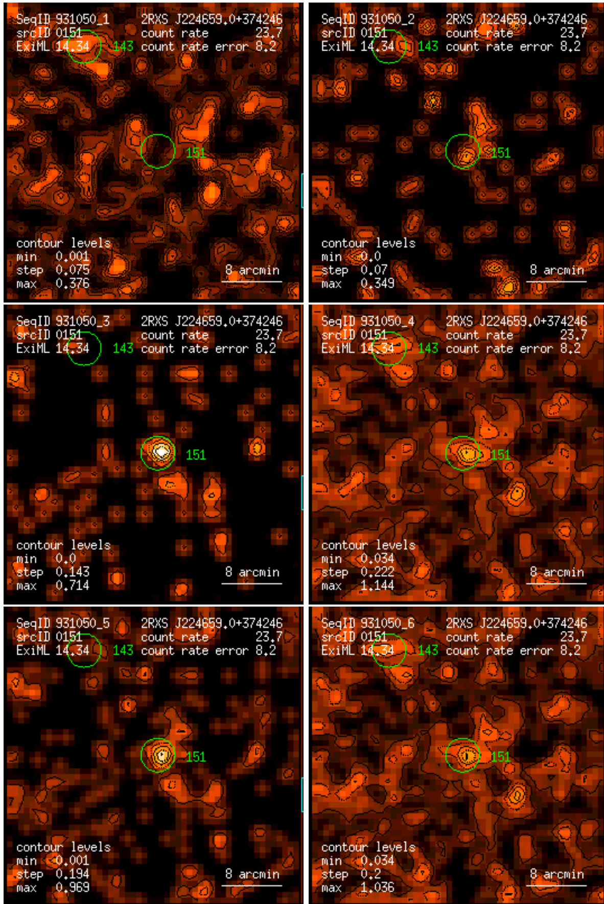
Figure 151: RASS 931050: detection 0151: band rate images, Gaussian filter: (1) PSPC channels 11 – 41, (2) 52 – 90, (3) 91 – 201, (4) 11 – 235, (5) 52 – 201, (6) 11 – 201. Broad band rates in counts/ks. Band rate contour levels in counts/ks/arcmin 2 .
