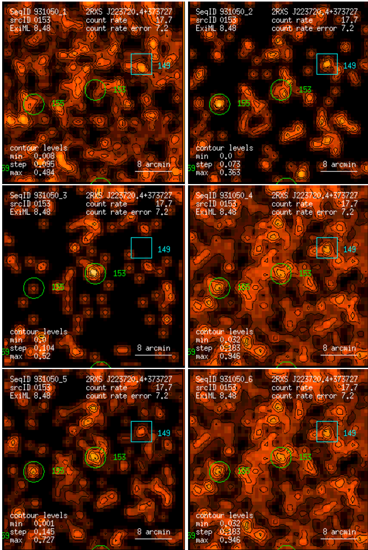
Figure 153: RASS 931050: detection 0153: band rate images, Gaussian filter: (1) PSPC channels 11 – 41, (2) 52 – 90, (3) 91 – 201, (4) 11 – 235, (5) 52 – 201, (6) 11 – 201. Broad band rates in counts/ks. Band rate contour levels in counts/ks/arcmin 2 .
