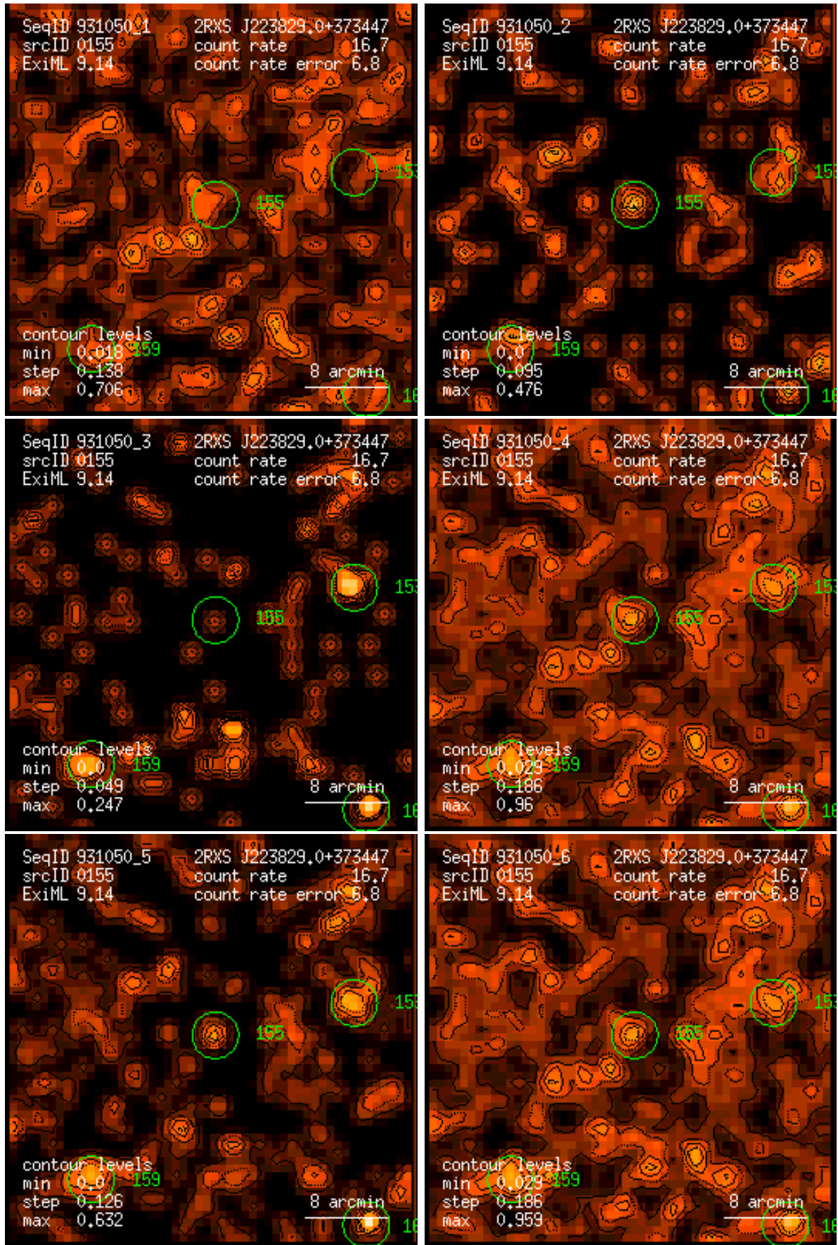
Figure 155: RASS 931050: detection 0155: band rate images, Gaussian filter: (1) PSPC channels 11 – 41, (2) 52 – 90, (3) 91 – 201, (4) 11 – 235, (5) 52 – 201, (6) 11 – 201. Broad band rates in counts/ks. Band rate contour levels in counts/ks/arcmin 2 .
