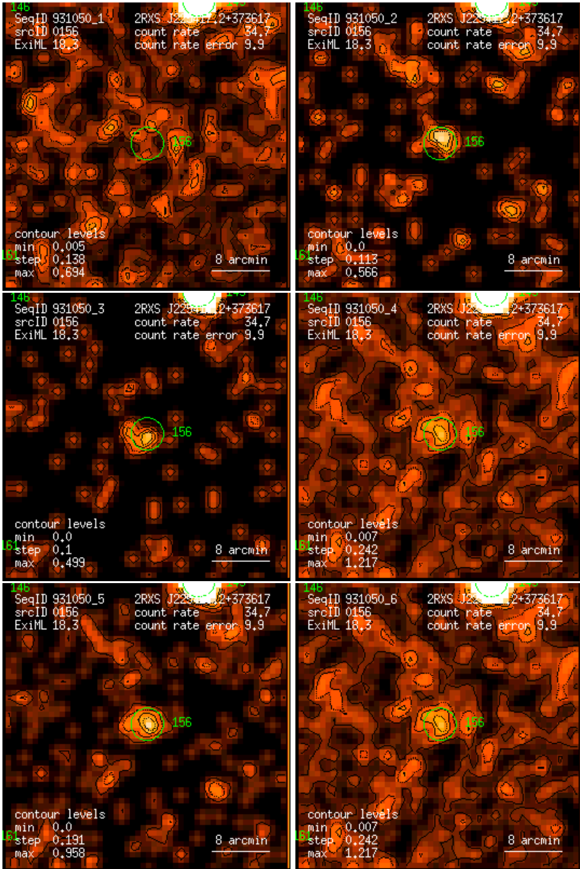
Figure 156: RASS 931050: detection 0156: band rate images, Gaussian filter: (1) PSPC channels 11 – 41, (2) 52 – 90, (3) 91 – 201, (4) 11 – 235, (5) 52 – 201, (6) 11 – 201. Broad band rates in counts/ks. Band rate contour levels in counts/ks/arcmin 2 .
