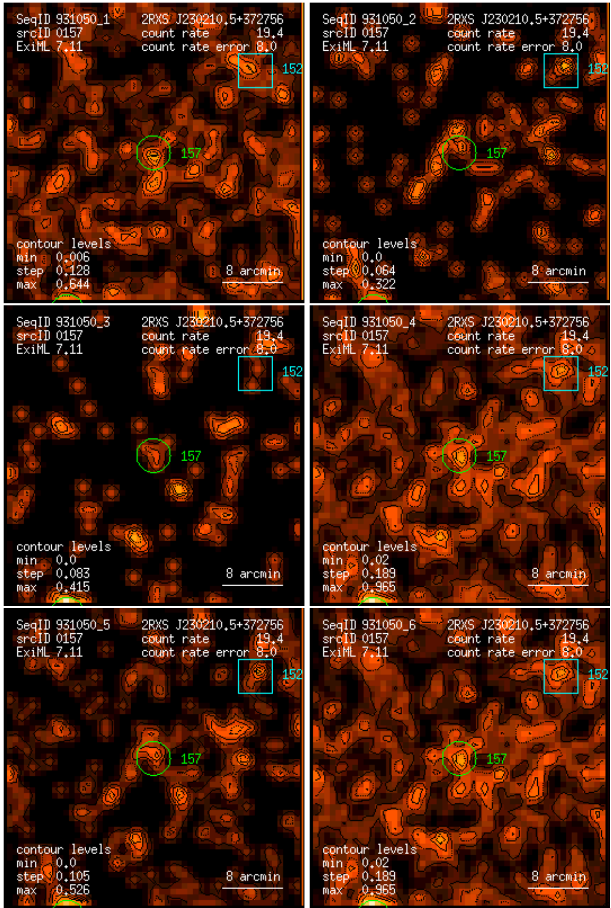
Figure 157: RASS 931050: detection 0157: band rate images, Gaussian filter: (1) PSPC channels 11 – 41, (2) 52 – 90, (3) 91 – 201, (4) 11 – 235, (5) 52 – 201, (6) 11 – 201. Broad band rates in counts/ks. Band rate contour levels in counts/ks/arcmin 2 .
