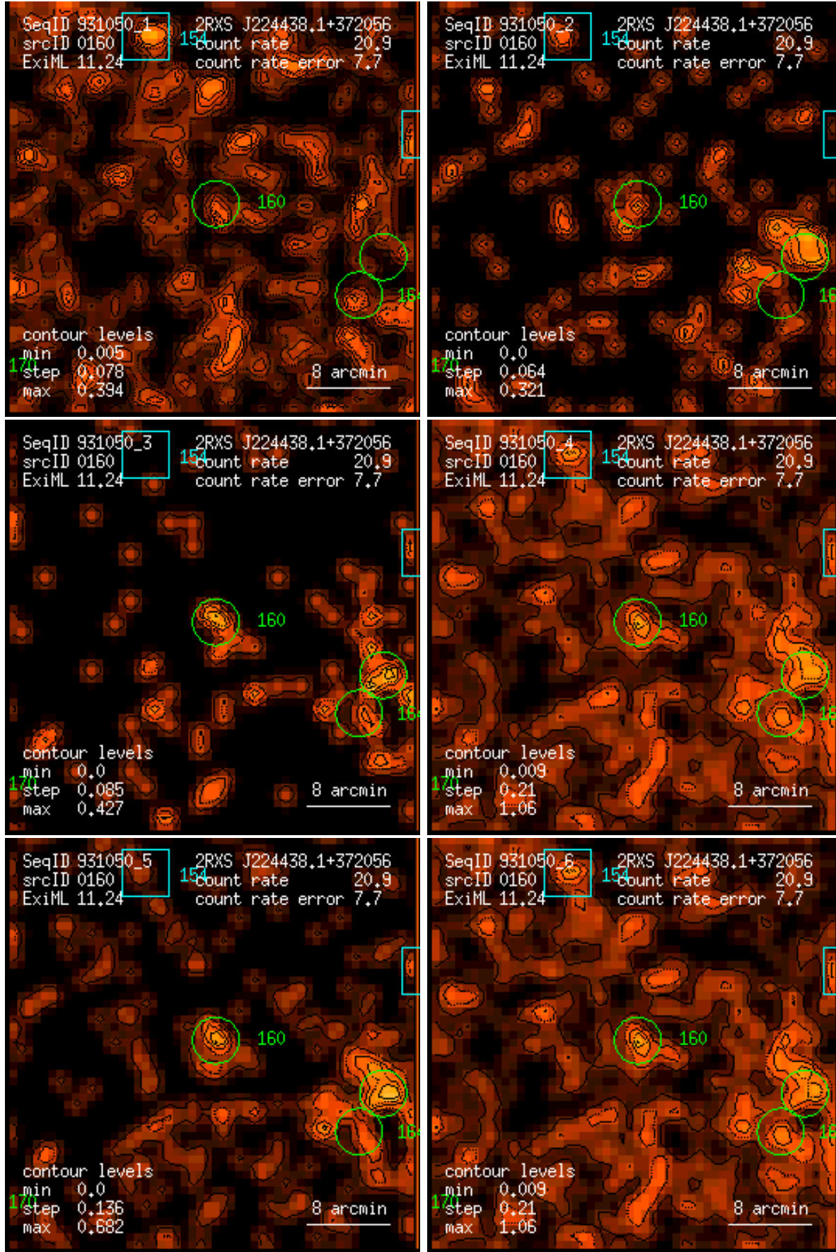
Figure 160: RASS 931050: detection 0160: band rate images, Gaussian filter: (1) PSPC channels 11 – 41, (2) 52 – 90, (3) 91 – 201, (4) 11 – 235, (5) 52 – 201, (6) 11 – 201. Broad band rates in counts/ks. Band rate contour levels in counts/ks/arcmin 2 .
